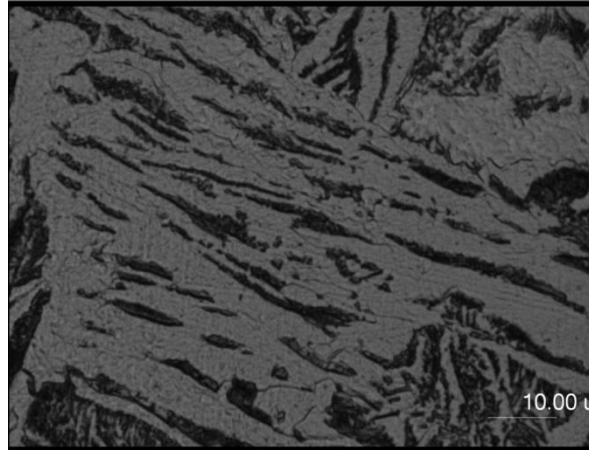
Figure 62: Steel 1018 Sample (Forged and Hammered) of Blade at Scale 10 \mu\text{m} and at 100X Magnification (after hammering).
