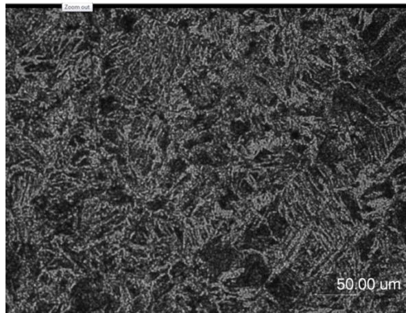
Figure 63: Steel 1018 Sample (Forged and Hammered) of Blade at Scale 50 \mu\text{m} and at 20X Magnification (after hammering).
