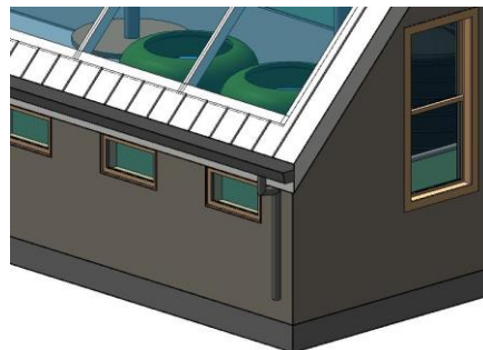
Figure 5: Rendering of the rainwater catchment system
