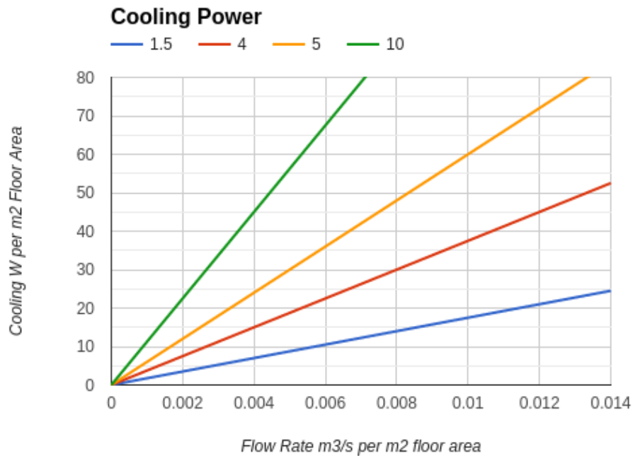
Figure 3.5.2(c) Chart to be used to determine cooling power
