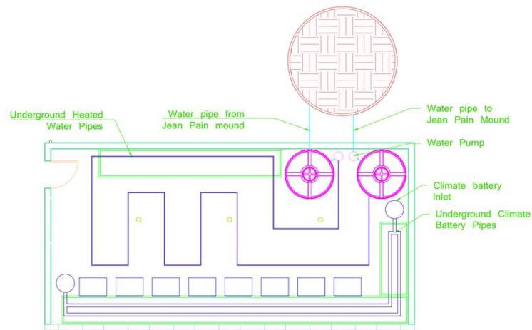
Figure 7: The underground layout of the heat conservation system
