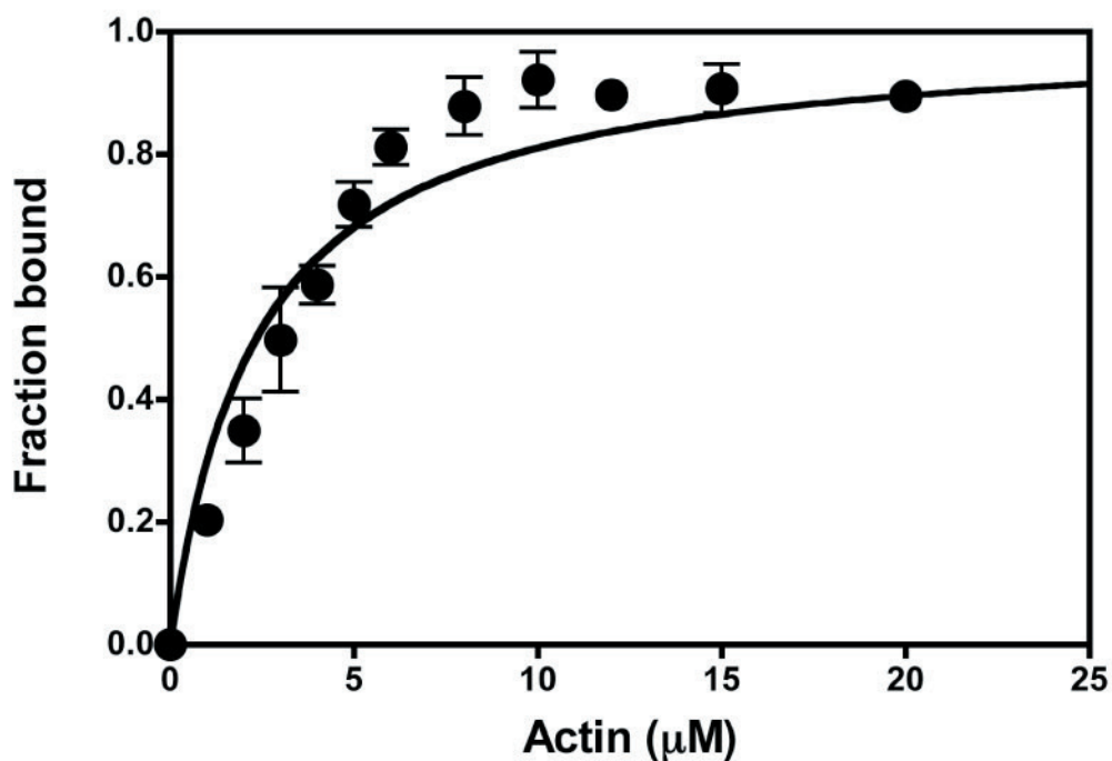
Fig. II-11. Actin binding activity of M9bIQ4 in the presence of ATP. Actin co-sedimentation assay of M9bIQ4 with actin was performed in the presence of 0.4 \mu\text{M} M9bIQ4, 1mM ATP, and various concentration (0 – 20 \mu\text{M} ) of actin. Pellet and supernatant were analyzed by SDS-PAGE. A, Coomassie staining of SDS gel. B, Fraction of bound M9bIQ4 with actin was plotted as a function of actin concentration. The data was fit to hyperbola ( v = B_{\text{max}}[\text{actin}]/(K_{\text{actin}} + [\text{actin}]) ), where B_{\text{max}} = 1 . K_{\text{actin}} of 2.33 \mu\text{M} is obtained. The error bars indicate S.D. for n = 3 from three independent preparations.
