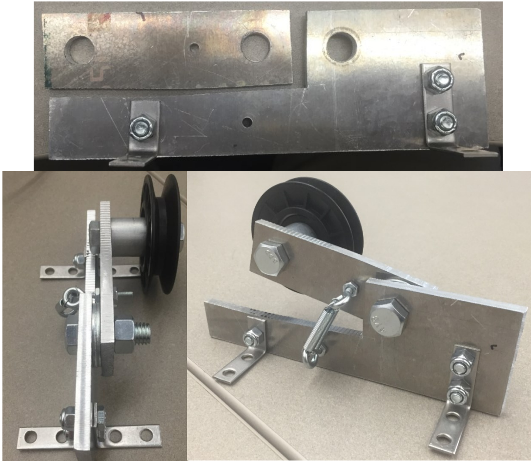
Figure 21 Final Tensioner Assembly
