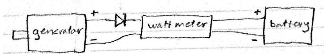
Figure 66 Battery charging test setup
