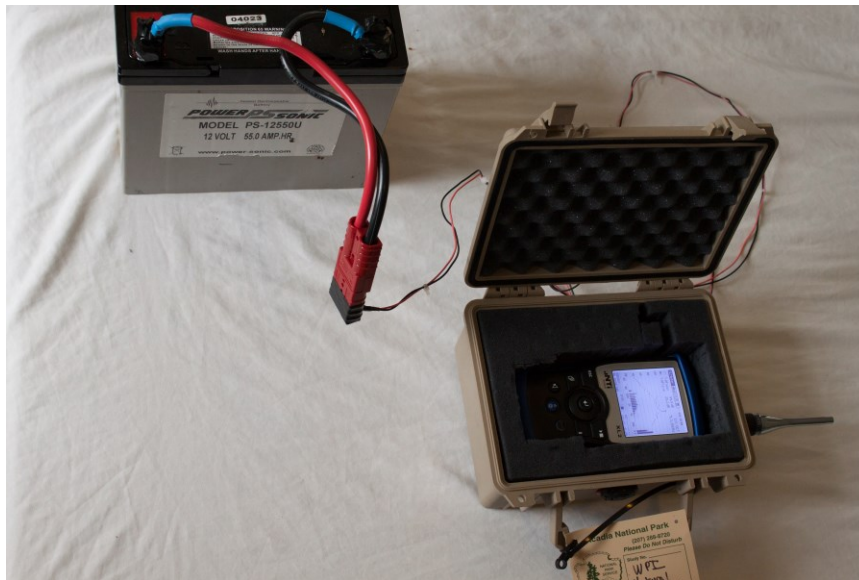
Figure 27: XL2 Inside Waterproof Case and Wired To Battery
