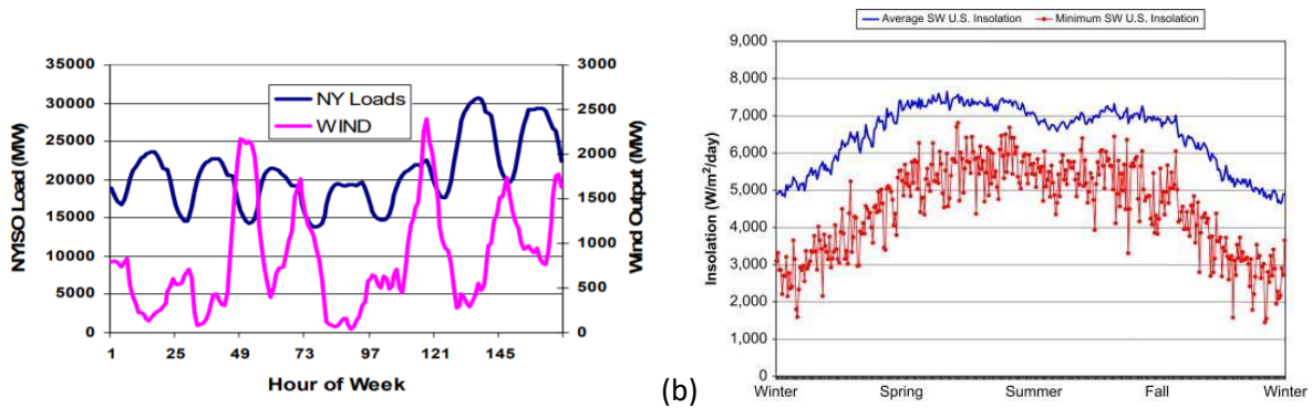
Figure 3. (a) Hourly Transience of Wind Power in New York 11 (b) Daily and Yearly Transience of Insolation in the American Southwest 12
