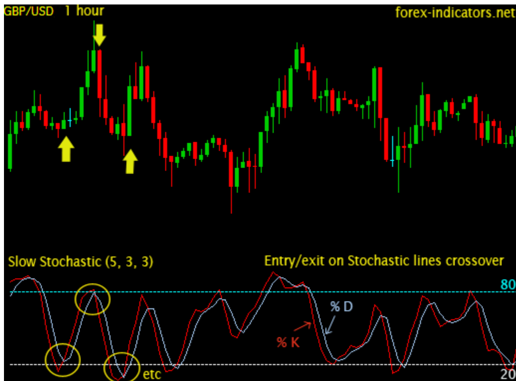
Figure 4.4b displays a stochastic indicator displaying entry and exit lines below price data.
