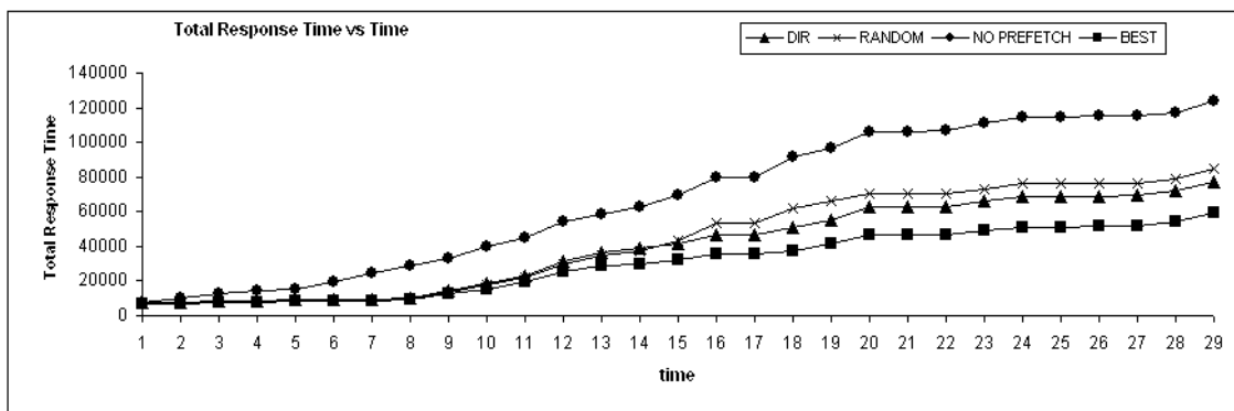
Figure 7.12: Response Time vs. Time for User A
