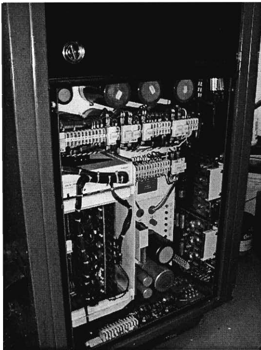
The inside of the BOSS 5 controller cabinet.
