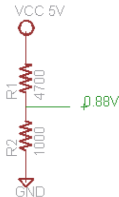
Figure 3.8: Schematic and calculations for a voltage divider
