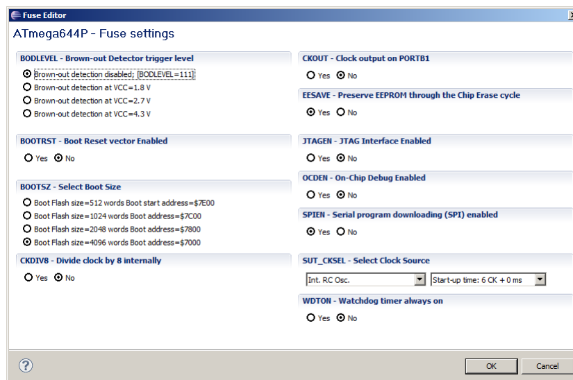
Figure C.5: Worksheet for setting internal fuses.
