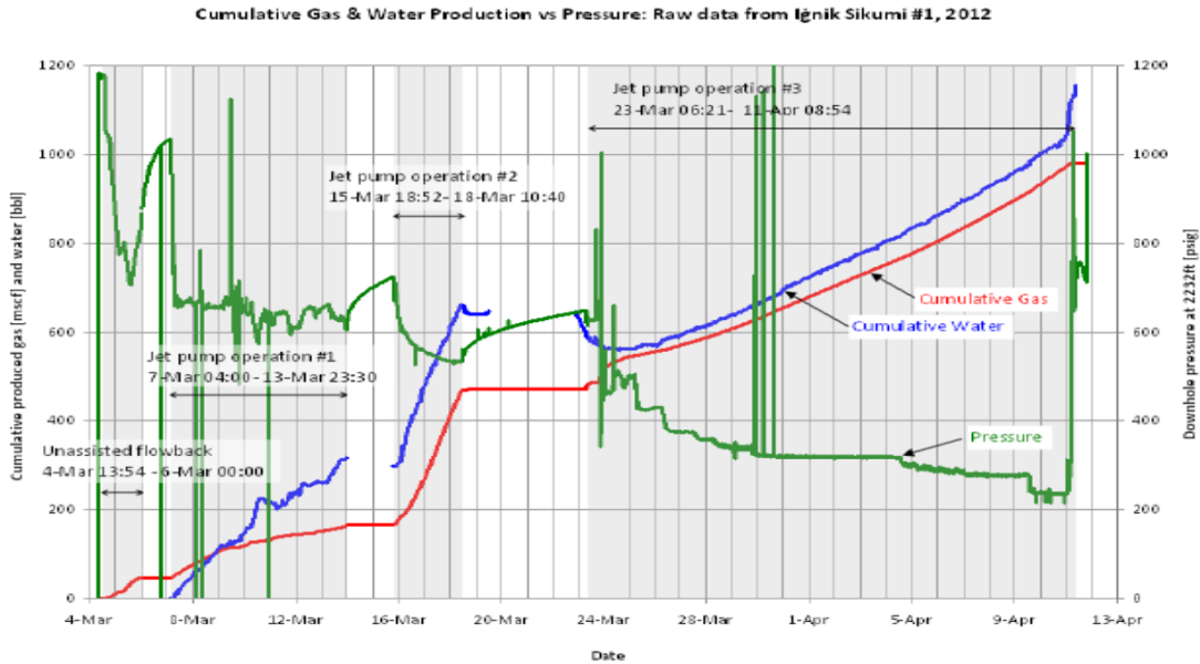
Figure 18: Flow back Data from Iğnik Sikumi
