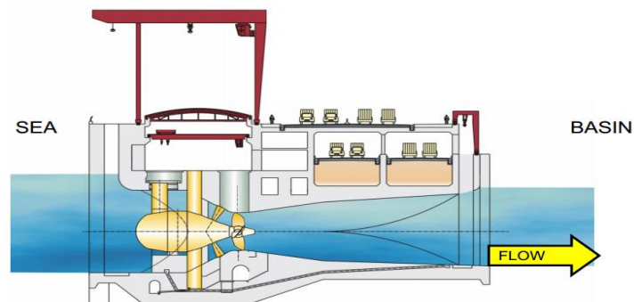
Figure 49: Sihwa Lake Tidal Station Motor
