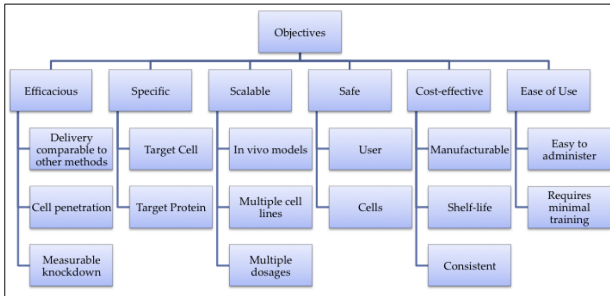
Figure 21: Objectives Tree
