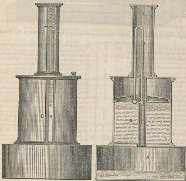
Tiffereau's Hydraulic Clock.
