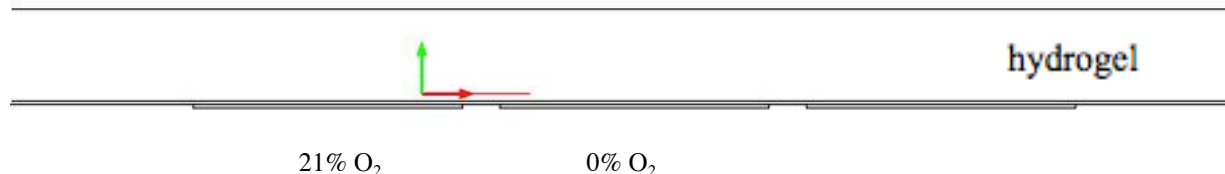
Figure 28: COMSOL model of cells in gel. The red axes show 200 micrometers above the membrane to simulate where the cells are in the hydrogel ( 1.97 \times 10^{-9} m 2 /s oxygen diffusivity in hydrogel, and 3.25 \times 10^{-9} m 2 /s oxygen diffusivity in PDMS)
