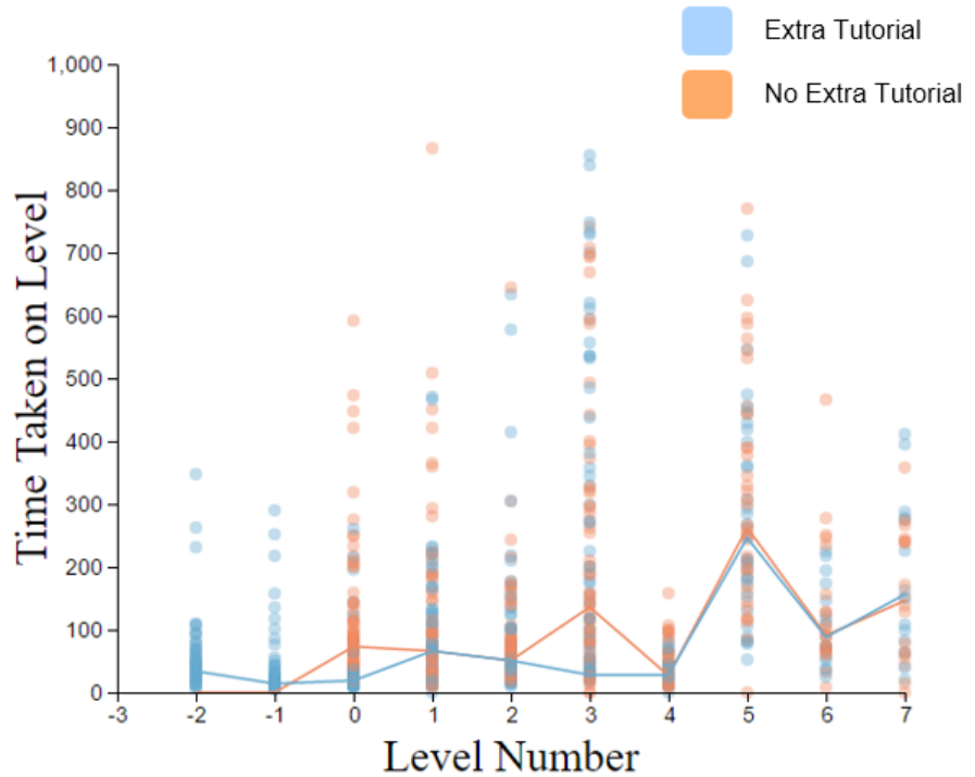
Figure 52. Level number vs. time taken graph. Image by Nick Chaput.
