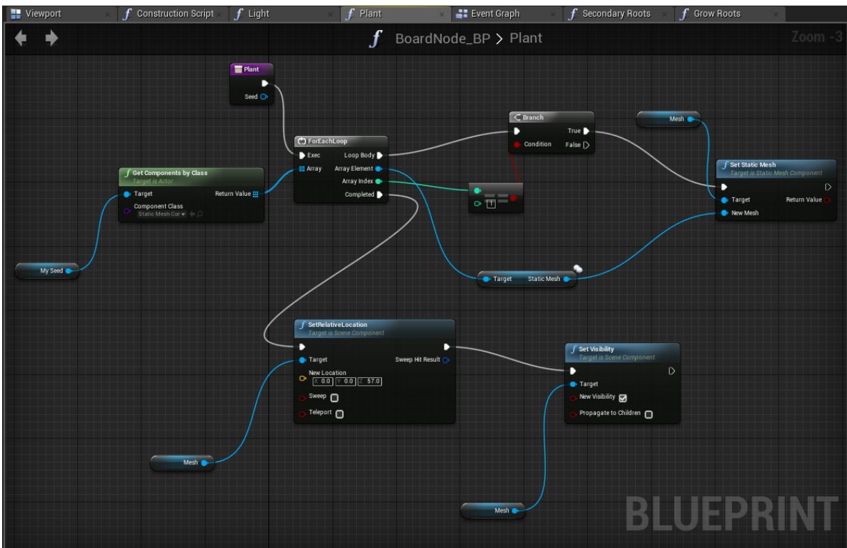
Figure 33: Blueprint Function Plant
