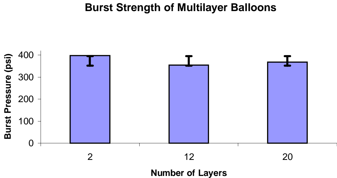
Figure 4.4 Burst strengths of 5mm 80/20 PET/Hytrel ® balloons with an increasing number of layers. Each value is the average of 10 balloons tested. Error bars signify one standard deviation.
