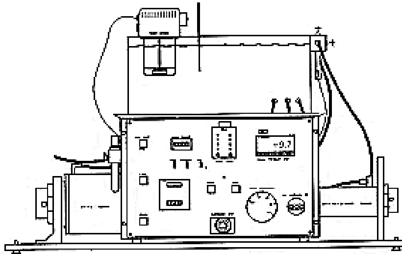
Figure 3.0.3 Heated water bath with pressurized lines to attach angioplasty balloons to for verification tests. 44
