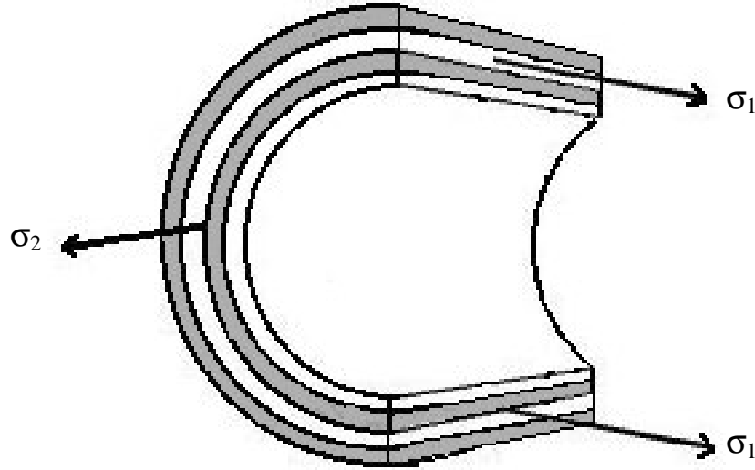
Figure 2.15 Sectional view of a multilayered, thin-walled cylinder experiencing circumferential ( \sigma_1 ) and longitudinal ( \sigma_2 ) stresses perpendicular to the broad faces of its layers.
