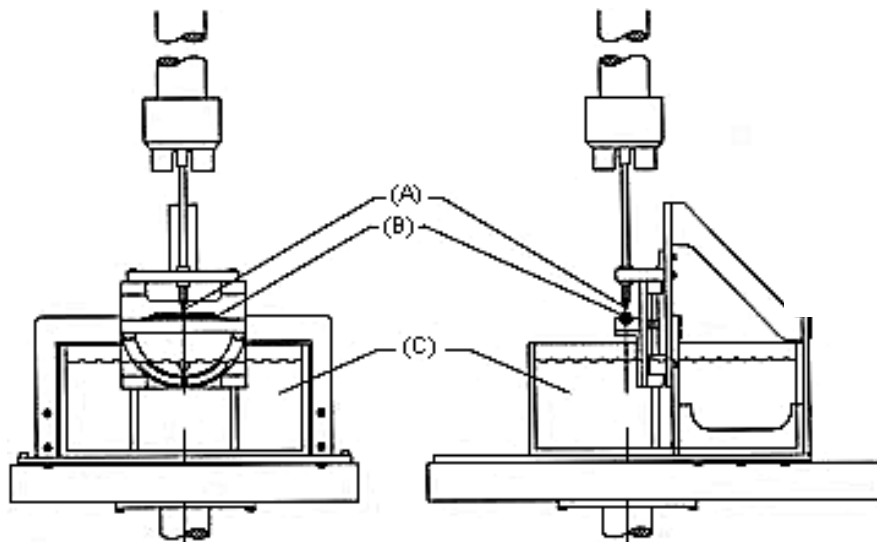
Figure 3.0.4 Fixture used with an Instron for puncture testing with (A) puncture tip, (B) balloon, and (C) heated water bath. 37
