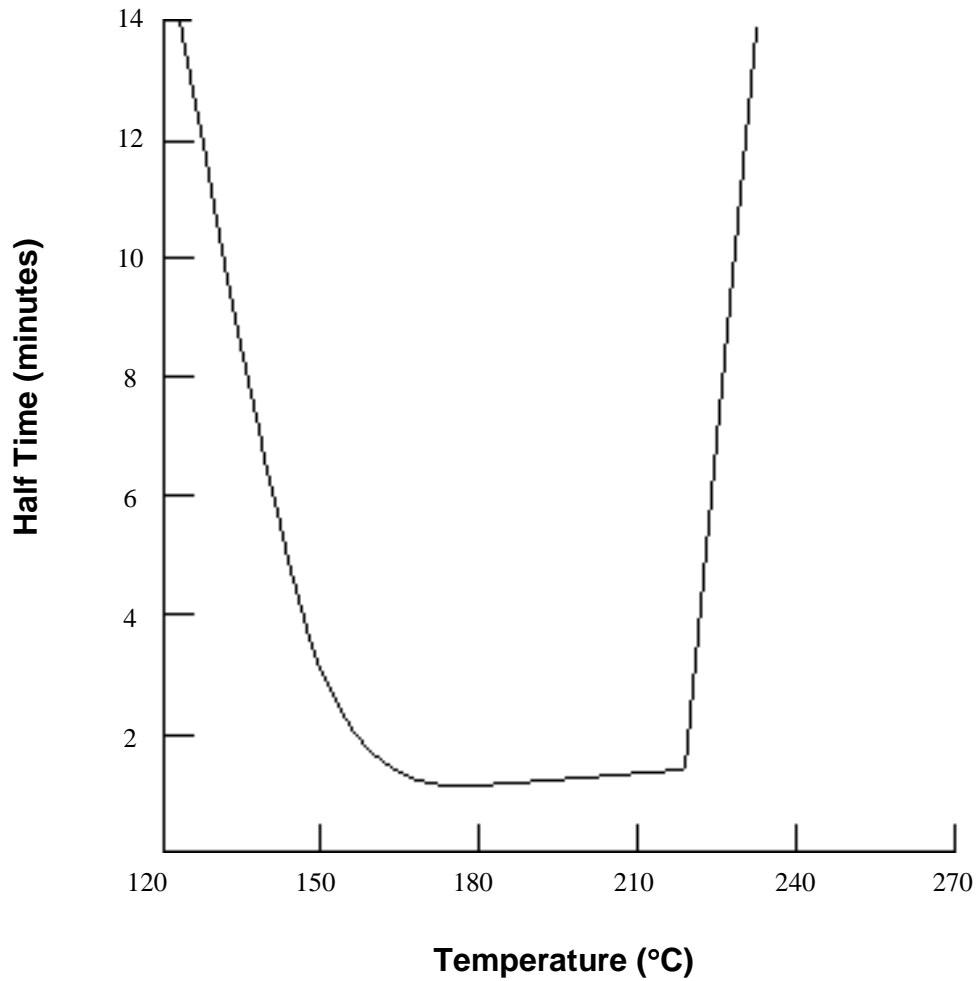
Figure 2.9 Half time crystallization rate versus temperature for PET. 20
