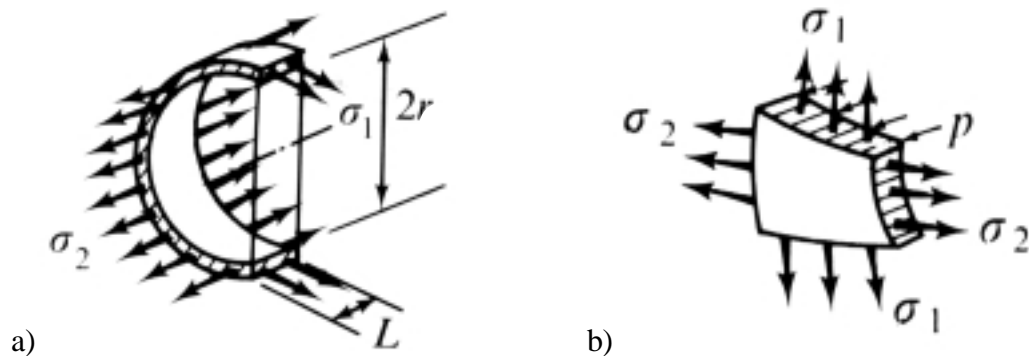
Figure 2.12 Applied stresses on a cylindrical thin-walled pressure vessel, where a) is a segment isolated from the vessel and b) is an element of the vessel wall in a state of biaxial stress. The normal stresses are \sigma_1 and \sigma_2 , p is the internal pressure of the vessel, r is the inside radius of the vessel, and L is the length of a longitudinal section of the vessel. 26
