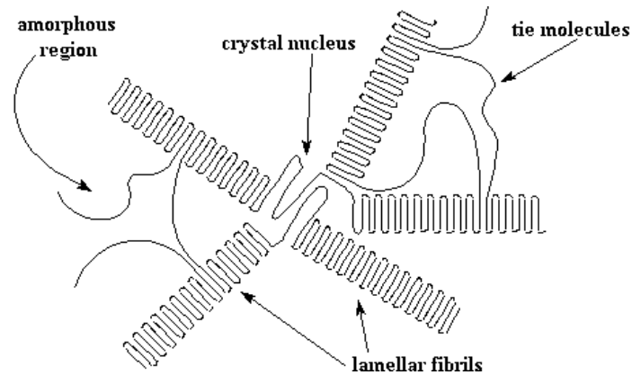
Figure 2.13 A polymeric spherulite composed of long molecules. 31
