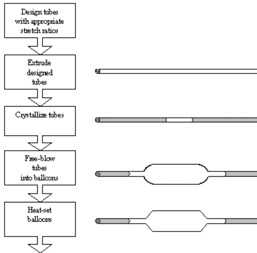
Figure 2.8 Illustrated flowchart of the processes involved in the fabrication and testing of balloons.
