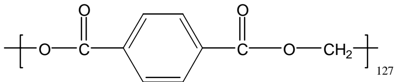
Figure 3.0.1 Chemical structure of Shell Cleartuf™ 8006
