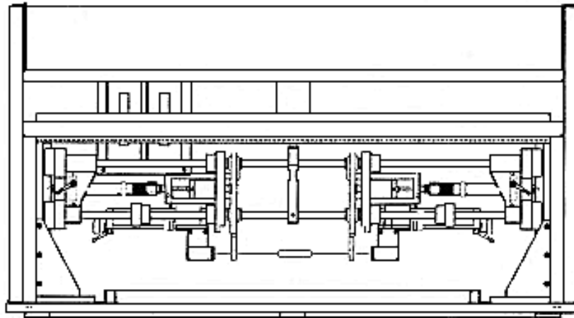
Figure 2.10 A typical machine used to free-blow angioplasty balloons. The balloon has been blown from a tube threaded between two grippers that was lowered into a glycerin bath and pressurized. 21
