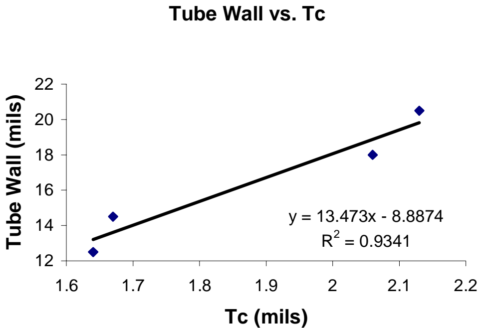
Figure 4.1 Thickness of tube wall versus double wall thickness (Tc) of the resulting balloon. Data used was obtained from twelve-layer balloons previously fabricated.
