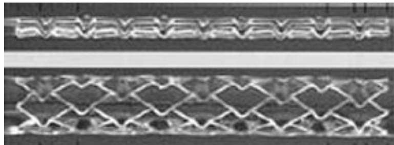
Figure 2.2 A NIR ® stent before (top) and after (bottom) expansion. 3
