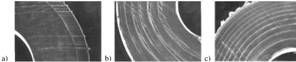
Figure 3.0.2 SEM micrographs of cross-sections of a) two-layer, b) twelve-layer, and c) twenty-layer 80/20 PET/Hytrel ® 5mm balloon tubes (150x)
