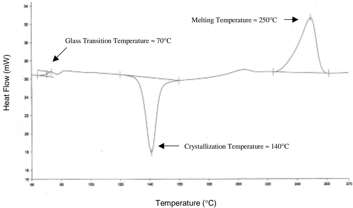
Figure 2.11 A Differential Scanning Calorimeter plot of an 80/20 PET/Hytrel ® extruded tube used in this investigation, with the PET transitions labeled. The tube was heated from 0 to 300 °C at 20 °C/min in a Perkin-Elmer DSC7.
