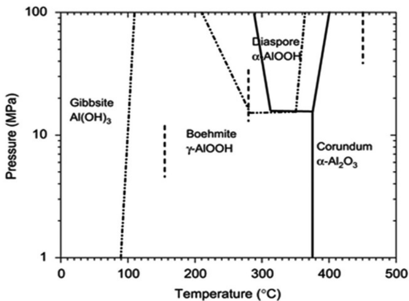
Figure 3. Phase diagram of boehmite and its transformations at various temperatures and pressures (Ghanizadeh et al., 2014).
