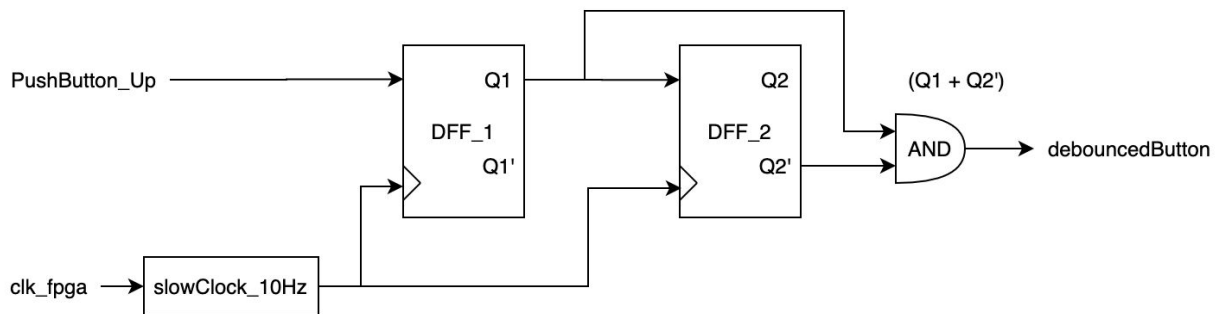
Figure 8: Block Diagram of Debounce Module
