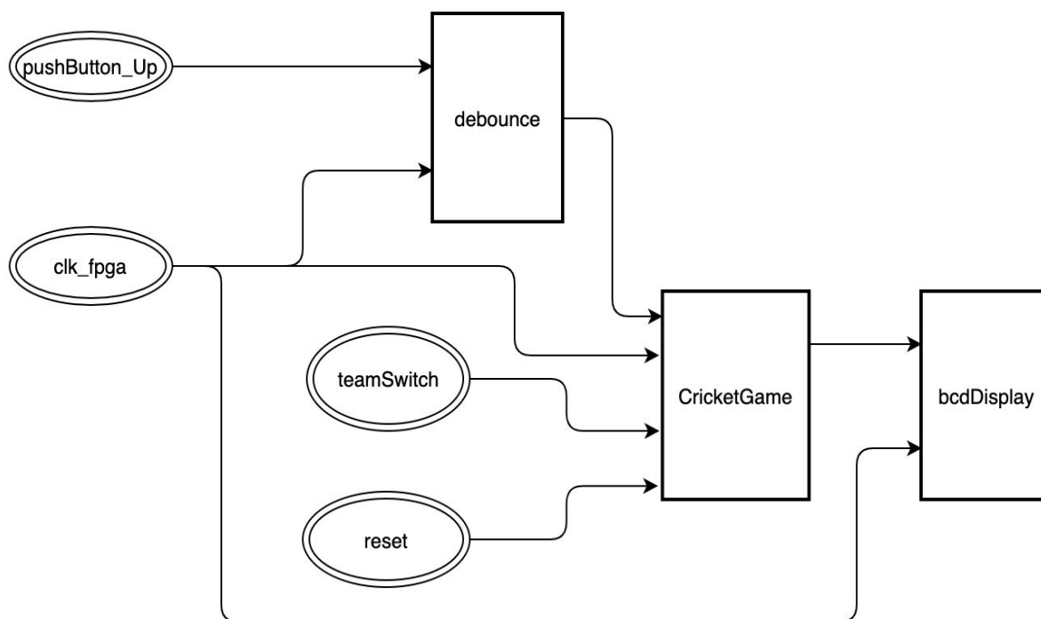
Figure 5: Functional Block Diagram of Cricket Top Module
