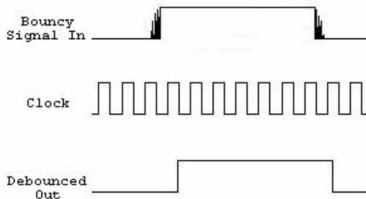
Figure 9: Timing Diagram for Generic Button Debouncing
