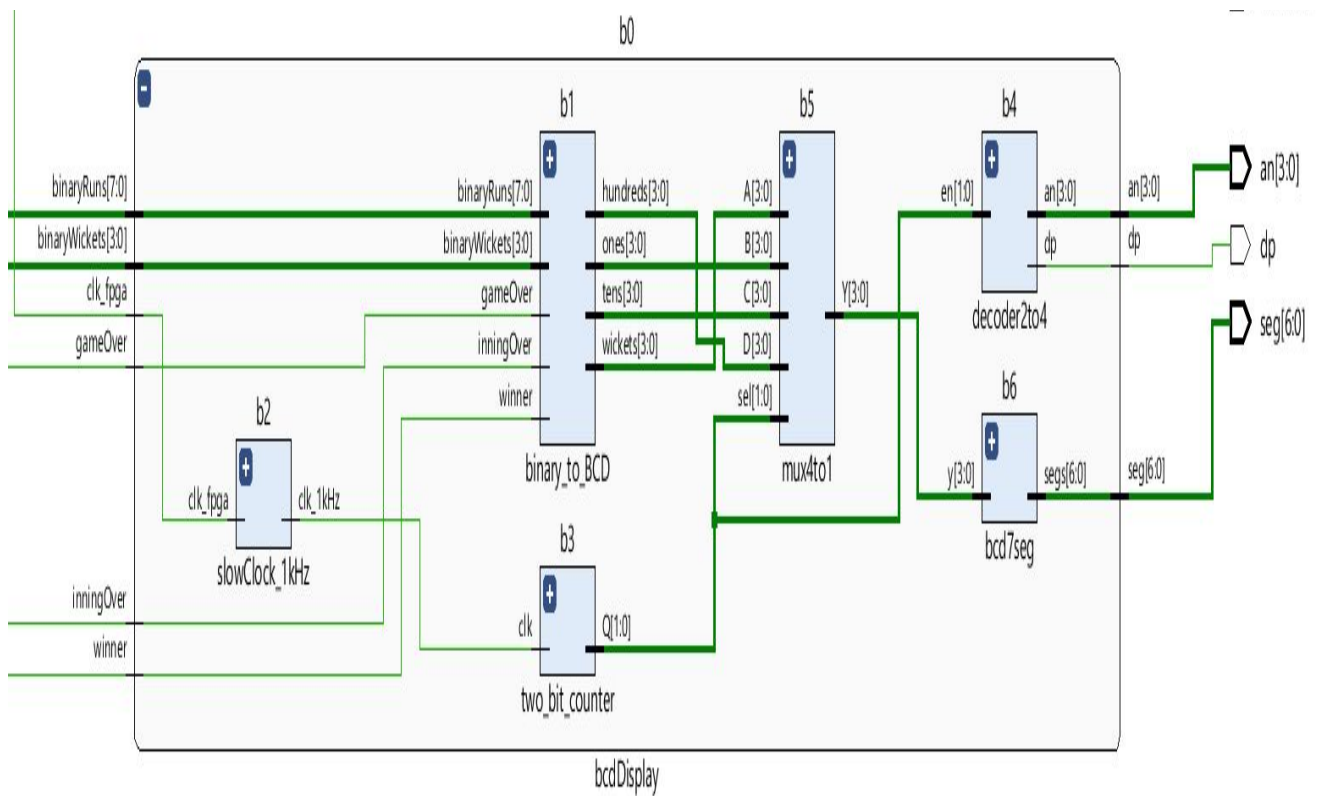
Figure 17: Verilog Schematic of Seven Segment Display
