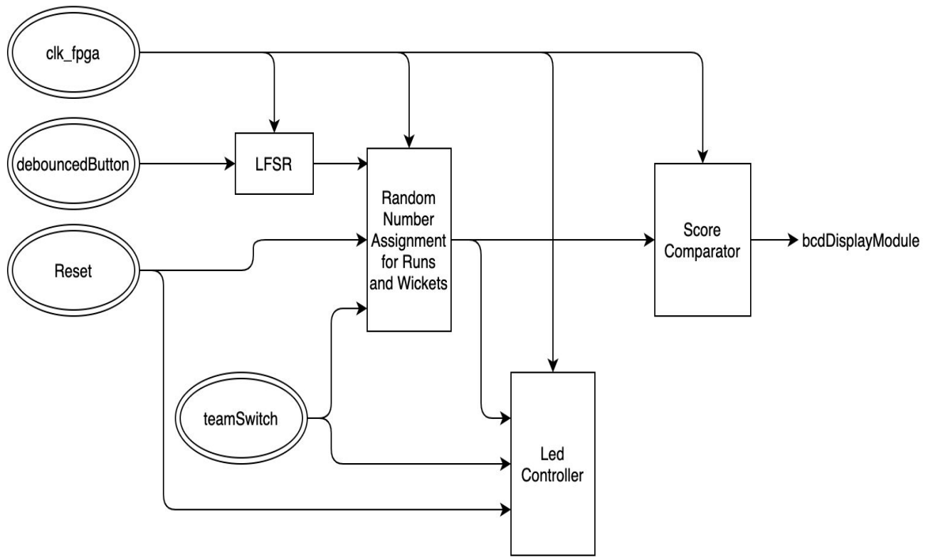
Figure 10: Block Diagram of Simplified Cricket Game Module
