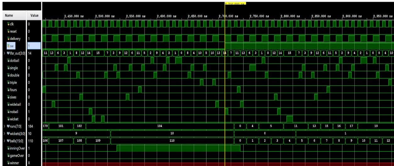
Figure 19: Timing Waveform - Switching Teams
