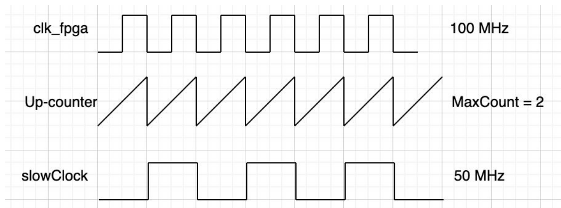
Figure 7: Timing Diagram to Generate Slow Clock from System Clock
