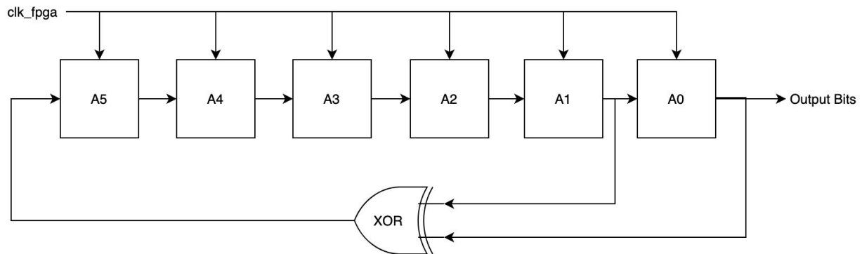
Figure 12: Block Diagram of LFSR Module for Random Number Generation [9]
