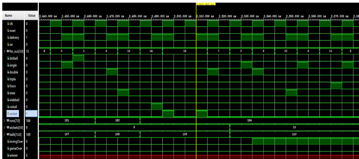
Figure 18: Timing Waveform - End of Team 1's Inning
