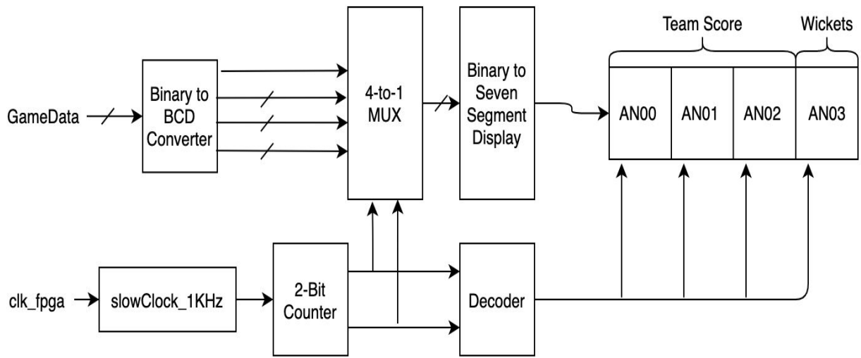
Figure 16: Block Diagram of Data from Game Module to Seven Segment Display [1]
