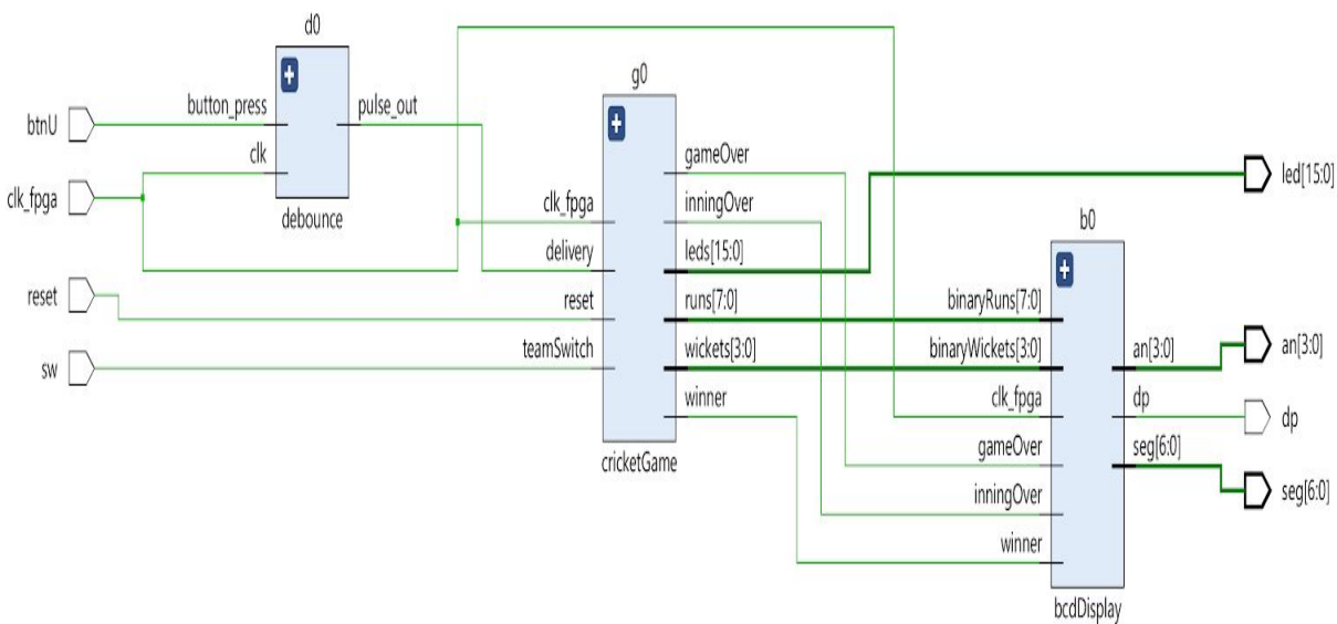
Figure 6: Verilog Schematic of Top Module
