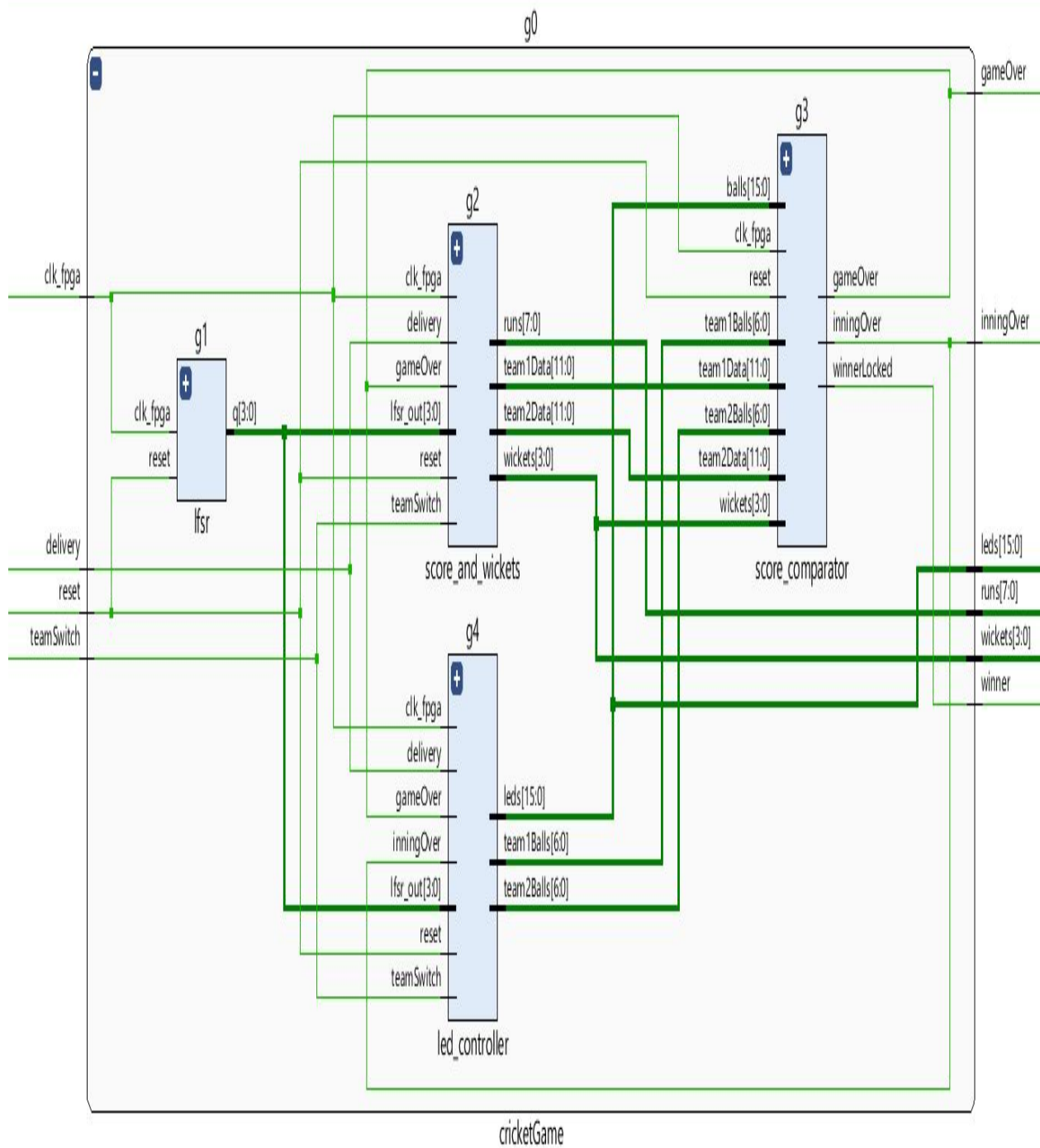
Figure 11: Verilog Schematic of Cricket Game Module
