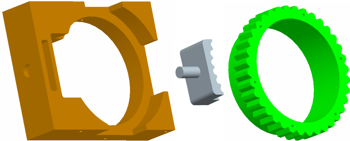
Figure 108 - Gear Brake
