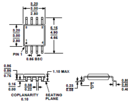
COMPLIANT TO JEDEC STANDARD 8 MO-187-AA Figure 58. 8-Lead Mini Small Outline Package [MSOP] (RM-8) Dimensions shown in millimeters
