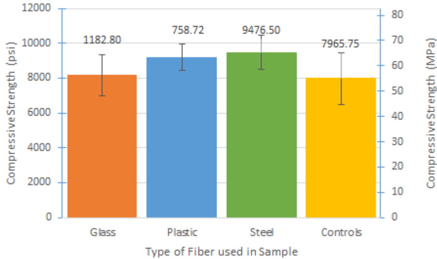
Figure 11: Comparison of compressive strength
