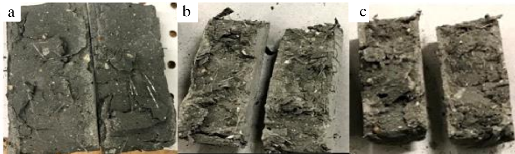
Figure 9: Cross sections of samples showing fiber distribution after split tensile test with a) steel fibers b) polymer fibers c) glass fibers
