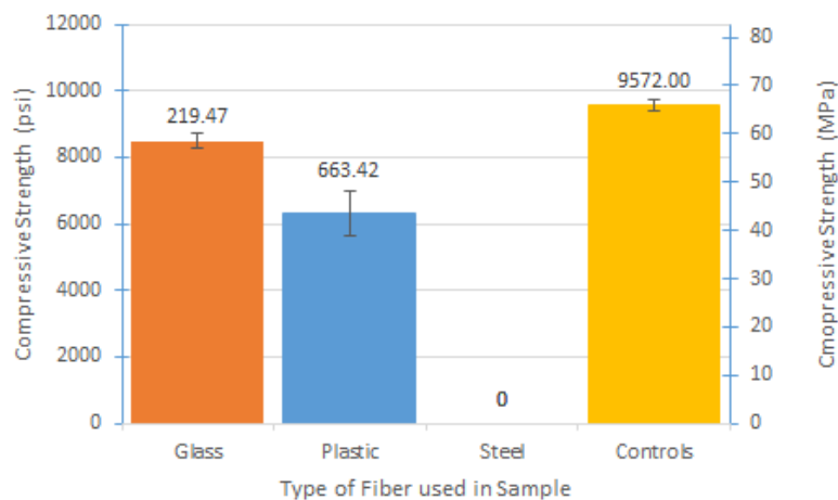
Figure 13: Comparison of compressive strengths after exposed to heat
