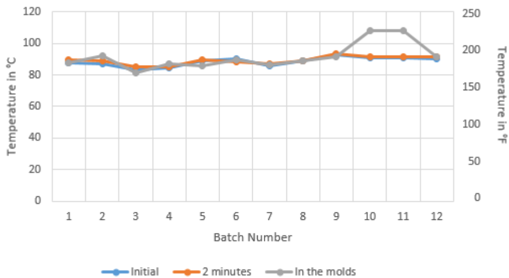
Figure 8: Graph showing that the temperature of each mix was mostly consistent except when the sand did not cool down enough
