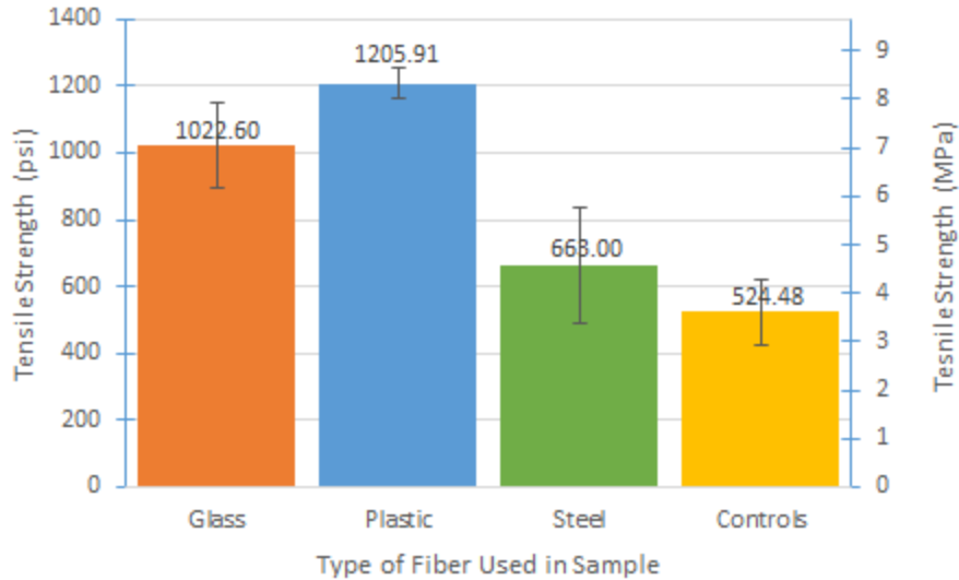
Figure 10: Comparison of the tensile strength
