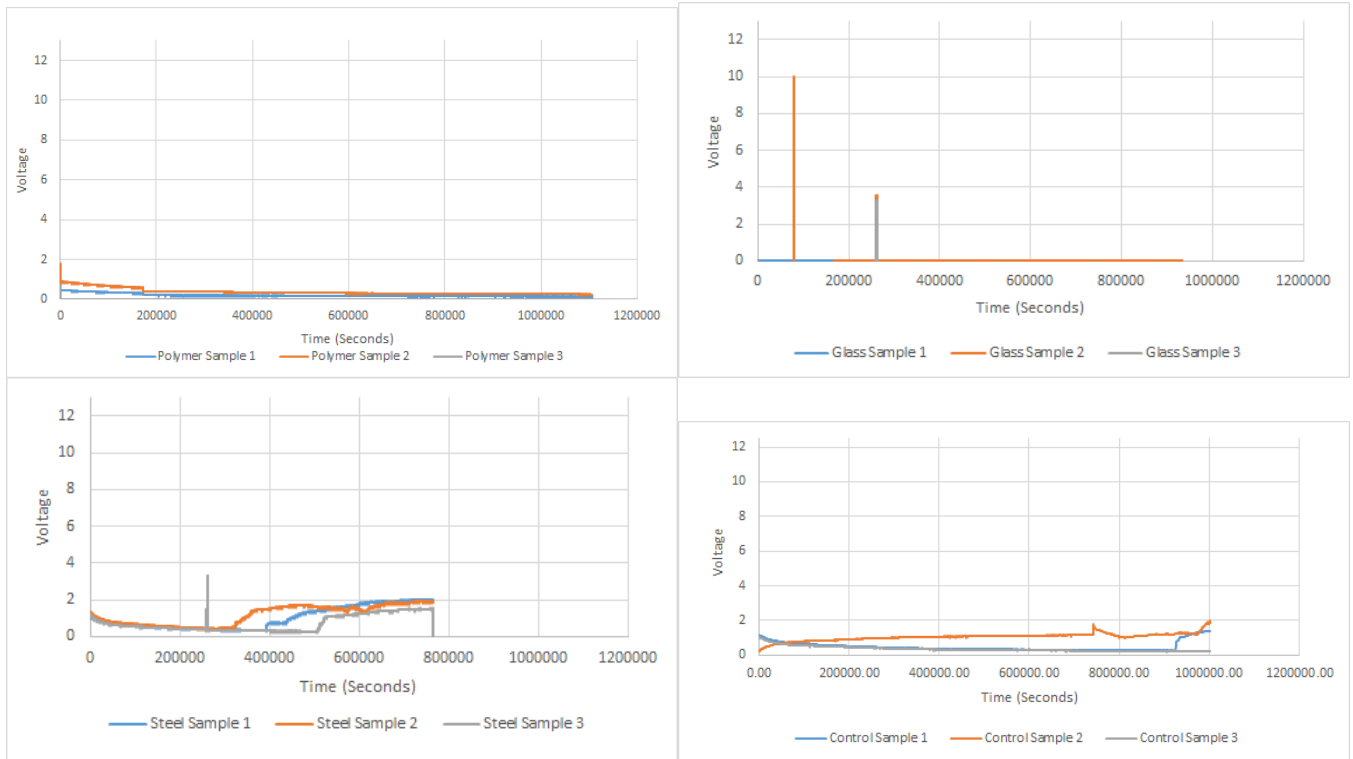
Figure 15: Corrosion testing graphs showing time (seconds) vs voltage for each of the samples
