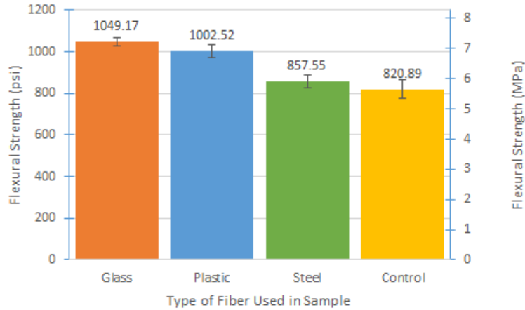
Figure 12: Comparison of the flexural strength
