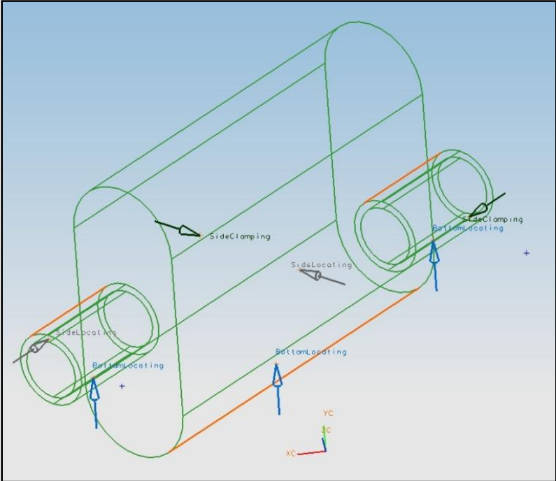
Fig. 24. Case 2 Supergraph.
