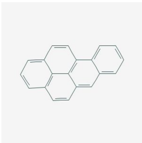
Figure 1: structure of of B[a]P
