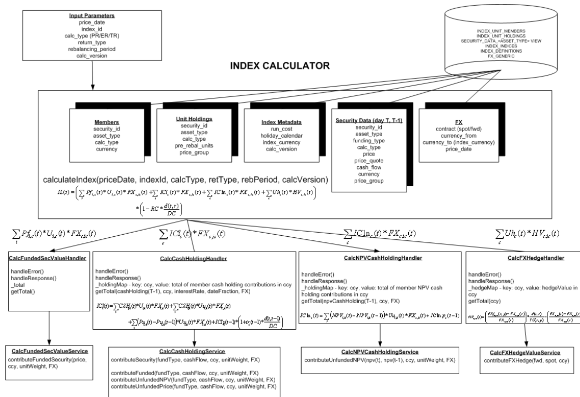
Figure 4 7 – DBIQ Index Calculator
