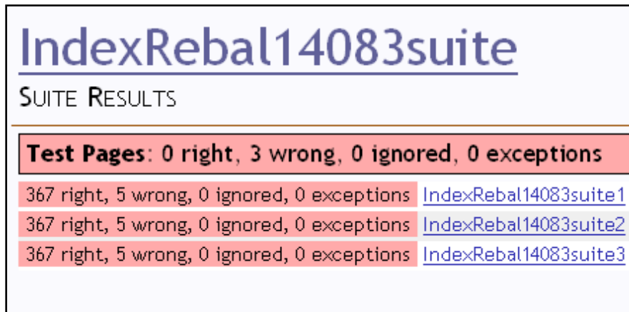
Figure 10 - A snapshot from a test suite showing the results from 3 tests
