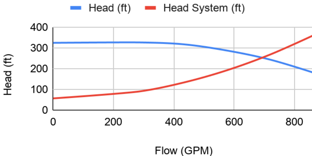
Figure 16: Operating Point Pump and System Characteristic Curve
