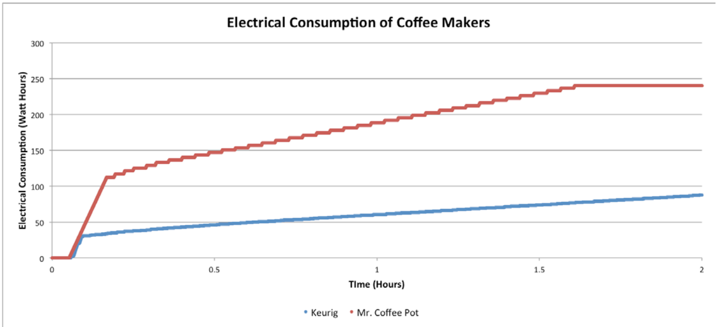
Figure 23: Keurig Watt-Hours
