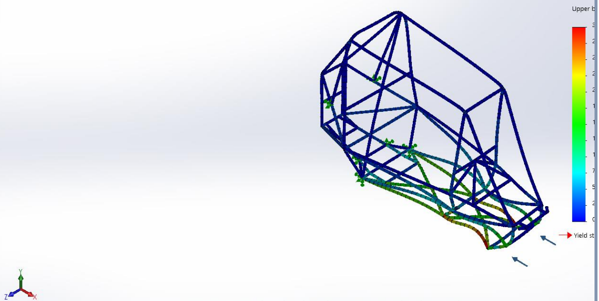
Model C18 2-6-17-Frontal Impact 2-Stress-Stress1
