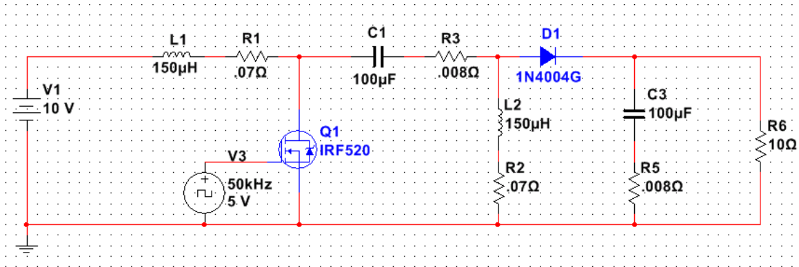
Fig 3.2 SEPIC Simulation
