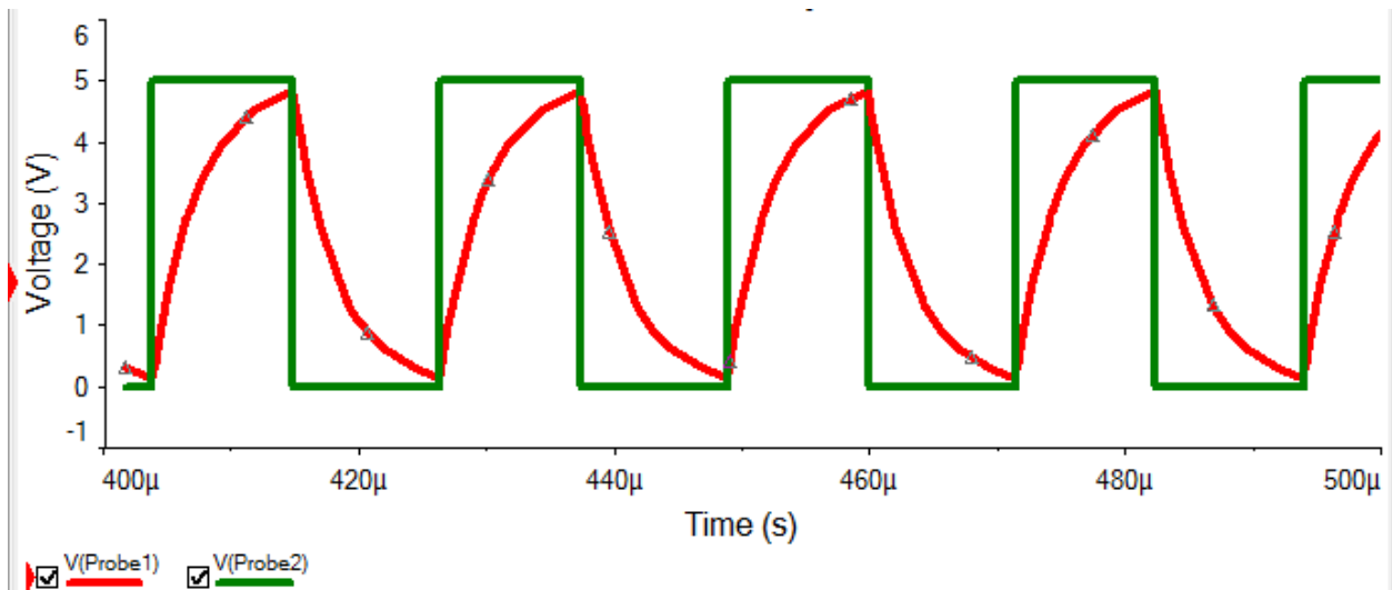
Fig 4.4 Graph of 555 and Triangle wave This is the output of the 555 with the triangle wave produced by the capacitor in lowpass.
