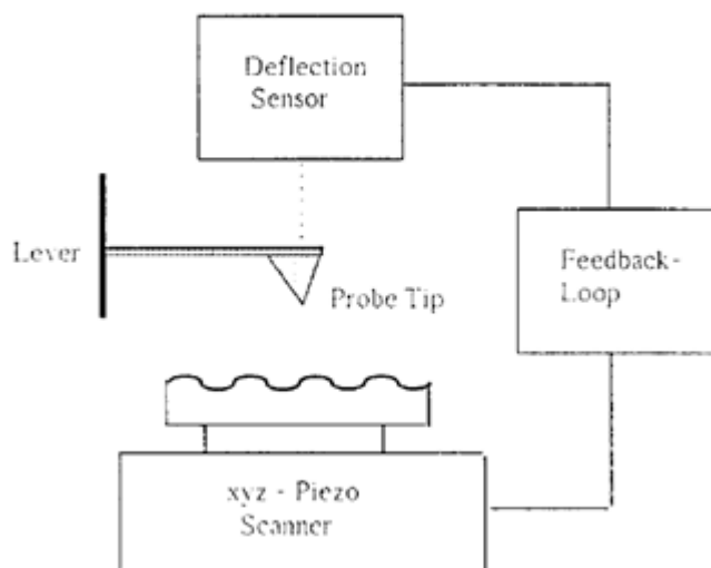
Figure 2: Basic principle of AFM. A sharp probing tip is mounted on a cantilever-type spring. The force between tip and sample causes cantilever deflections which are monitored by a deflection sensor. While scanning the samples a feedback-loop can keep the deflection constant (Meyer, Atomic Force Microscopy, Progress in Surface Science, Vol. 41, pp, 3-49, 1992)
