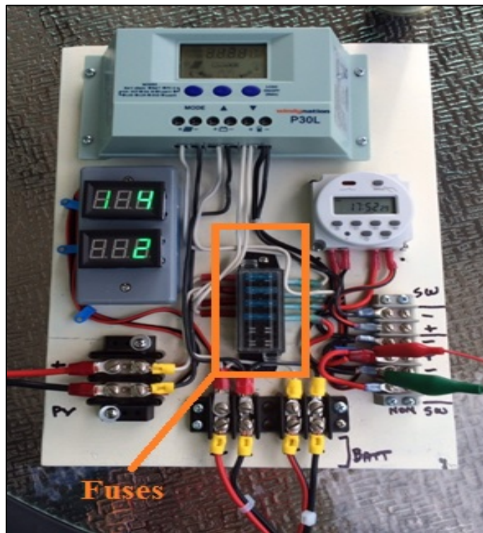
Figure 55 - Fuses
