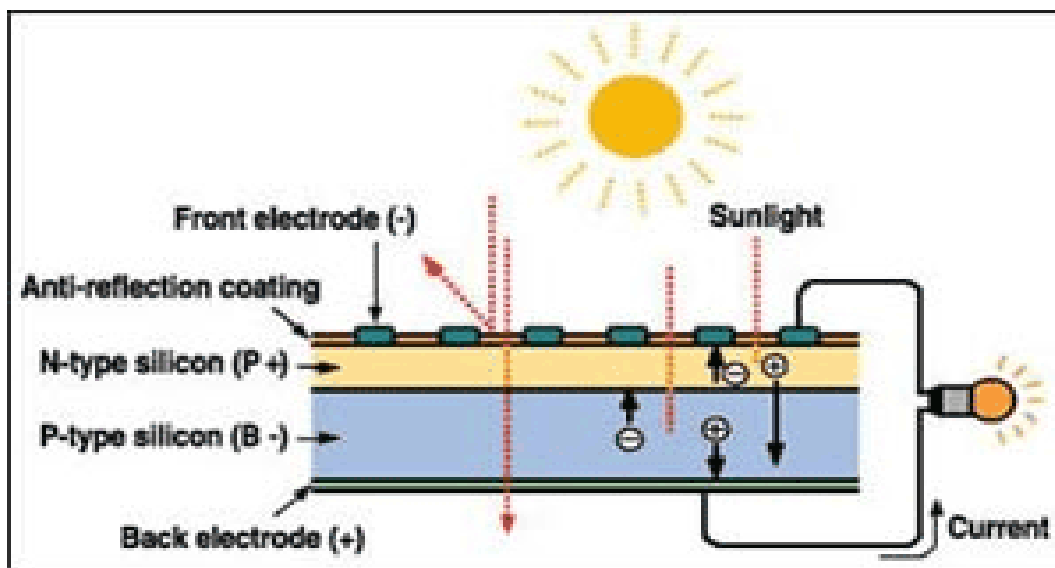
Figure 5 - Basic photovoltaic cell operation
