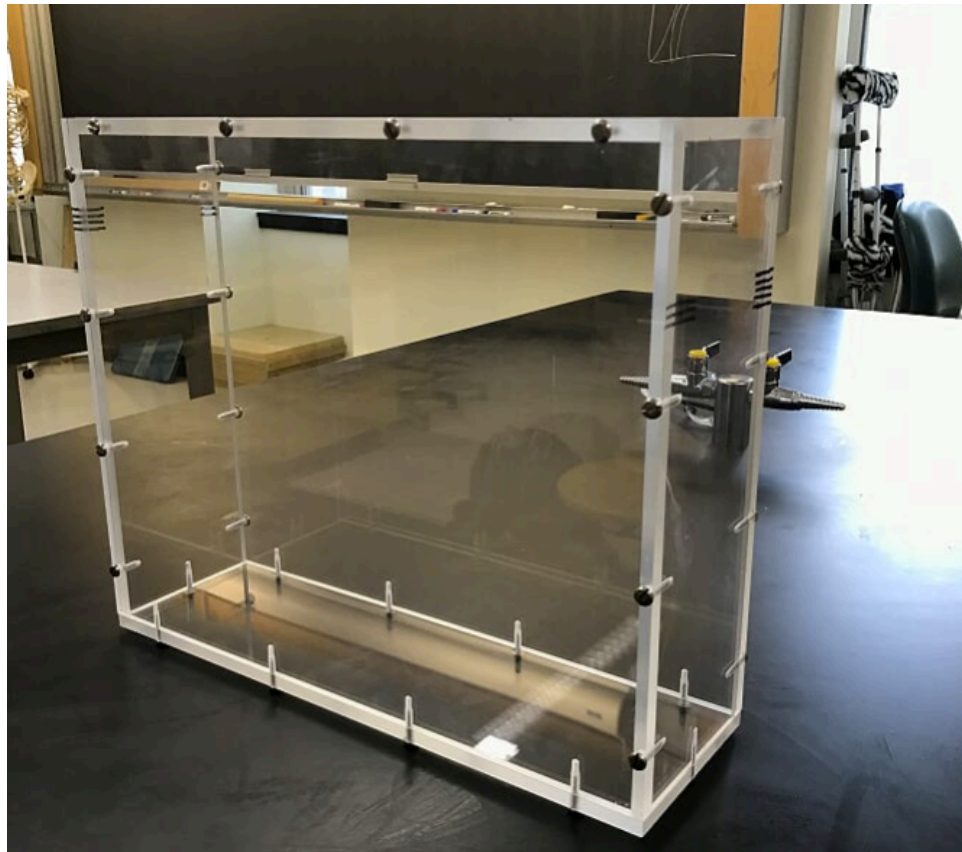
Figure 18 Plexiglas box (12x14.5x4 in) built to mold the organs with silicone
