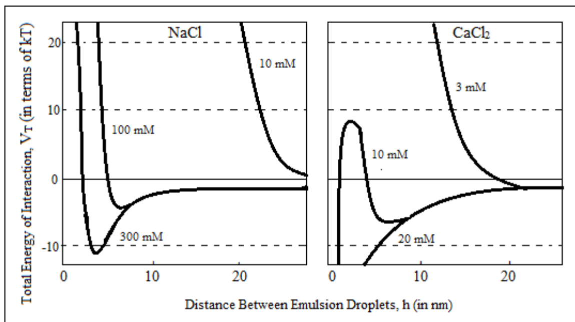
Figure 2.4 Energy diagrams for bitumen-in-water emulsions in the presence of NaCl and \text{CaCl}_2 (Israelachvili 1992)
