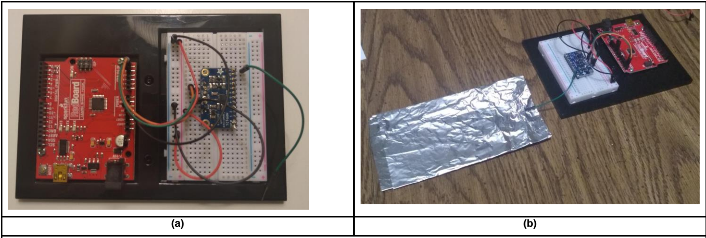
Figure 5.2.3: Touch Sensor Test Circuit.
