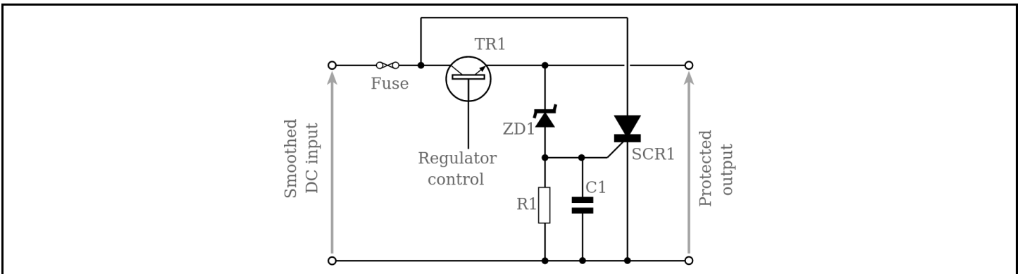
Figure 4.2.14: SCR Crowbar Circuit
