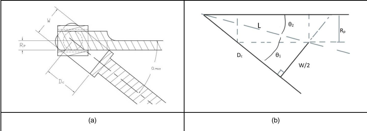
Figure 4.1.9: Cross sectional geometry of platform U-Joint
