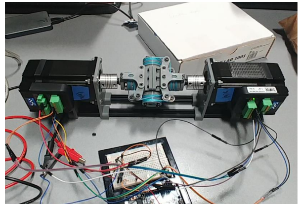
Figure 5.1.3: Stepper driven test fixture
