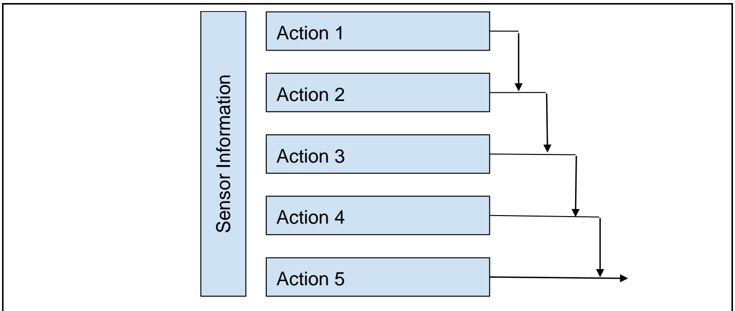
Figure 4.3.7: Diagram of a Subsumption System
