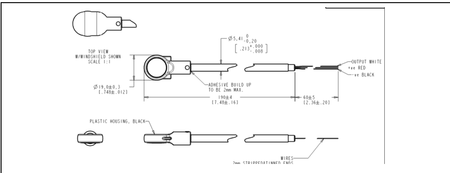
Figure 4.2.5: FB-EM-30346-000 Microphone [27]
