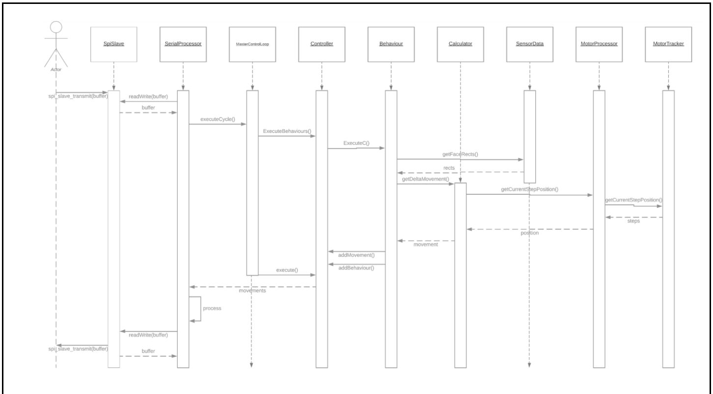
Figure 5.3.2: Sequence Diagram
