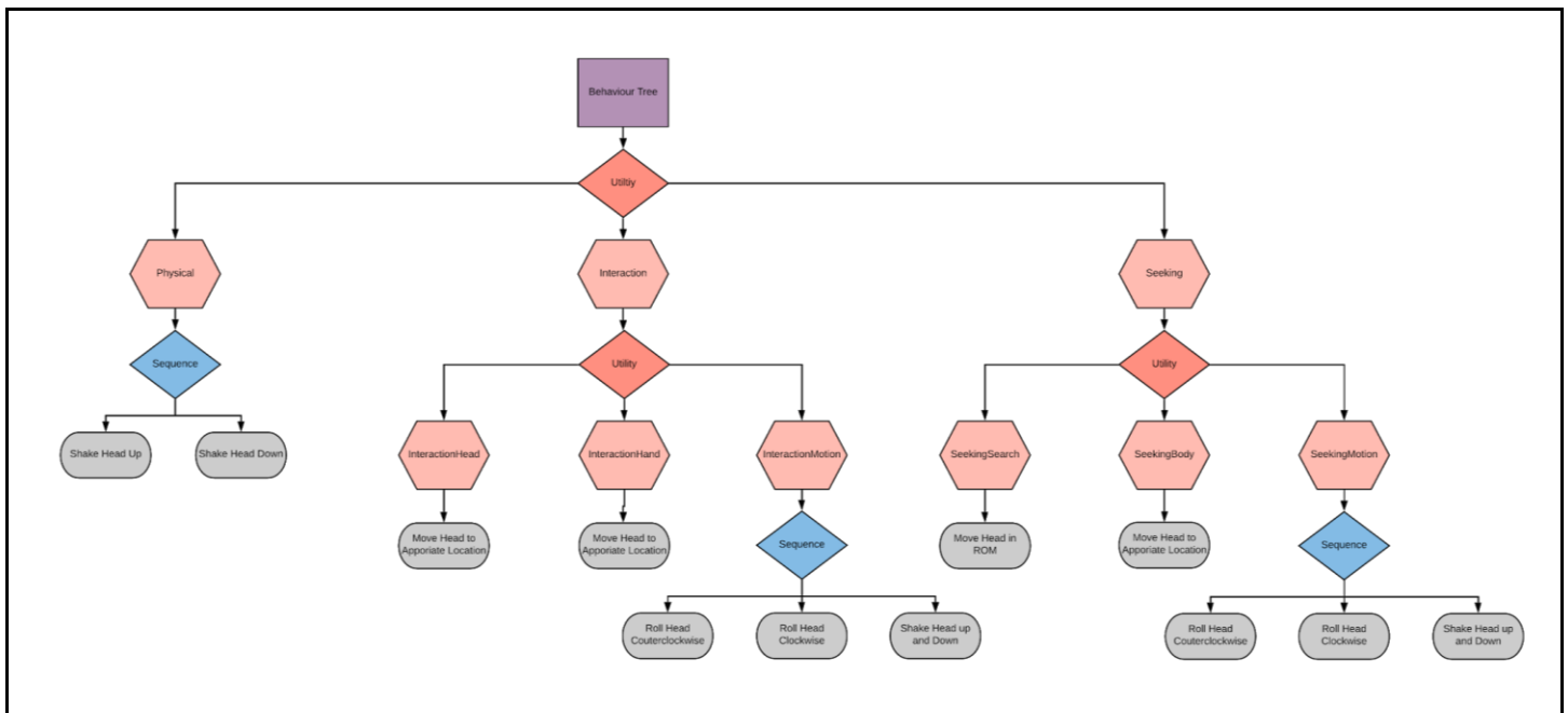
Figure 4.3.11: Behavior Tree Diagram
