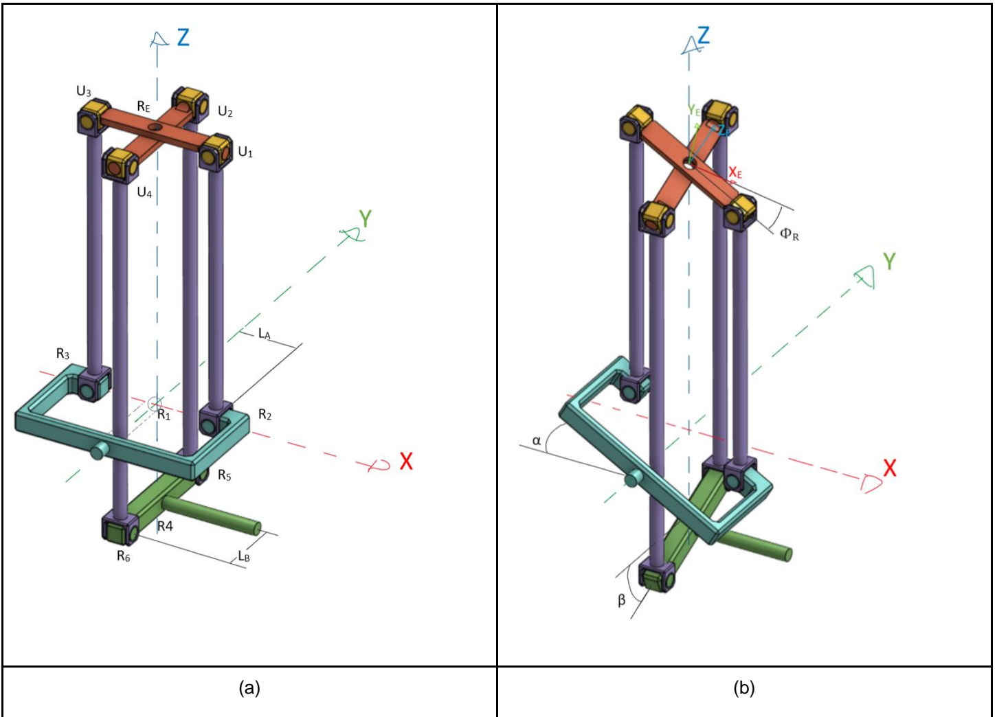
Figure 4.1.7: Labeling conventions of the u-joint platform
