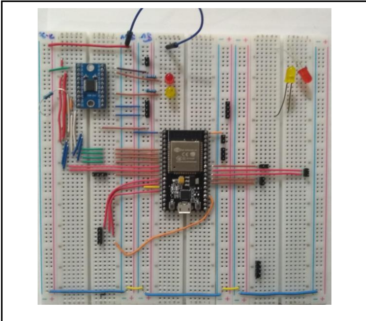
Figure 5.2.4: Motor Test Circuit
