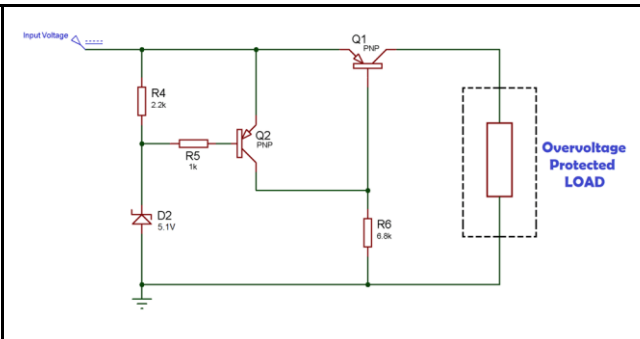
Figure 4.2.13: Overvoltage Protection Circuit [18]
