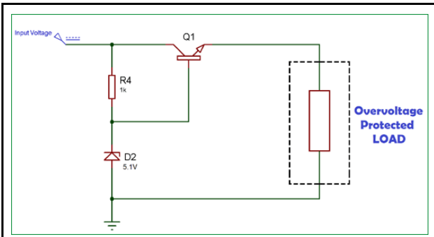
Figure 4.2.12: Zener Regulator Circuit [18]
