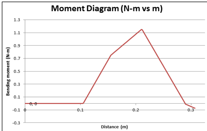
Figure 40: Moment diagram of the rocker
