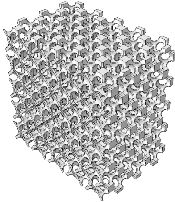
Figure 7: Steel Foam Structure 2
