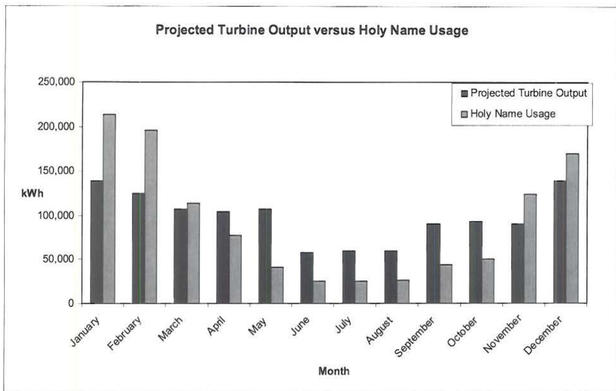
Figure 1: Projected Turbine Output versus Holy Name Usage
