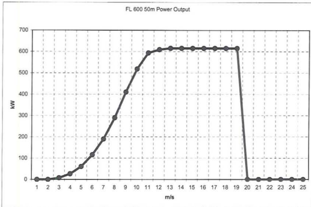
Figure 50: FL600 50m Power Output Curve
