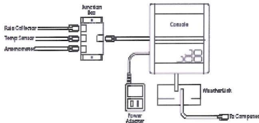
Weather Wizard III Connection Diagram
