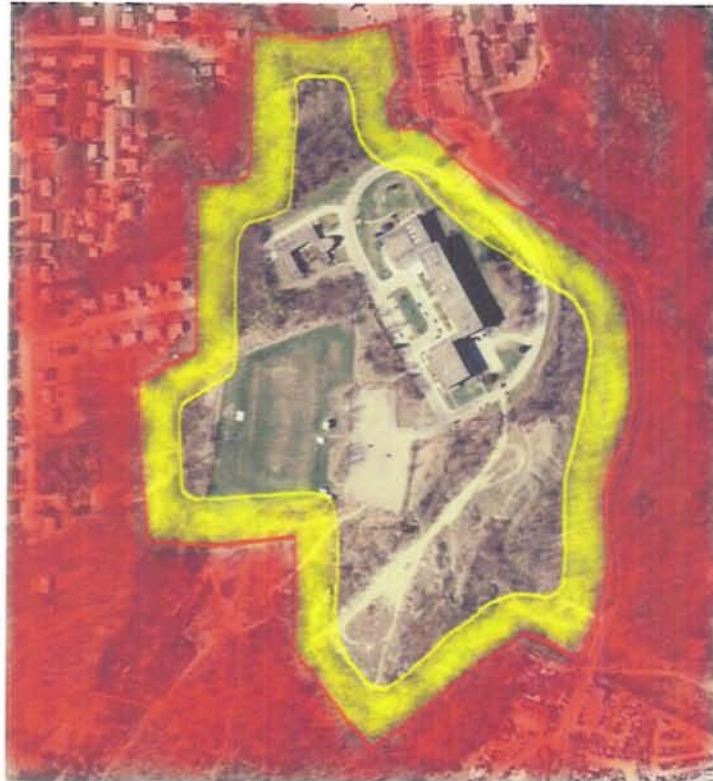
Figure 40: Available Land for Turbine with Property Line Restrictions
