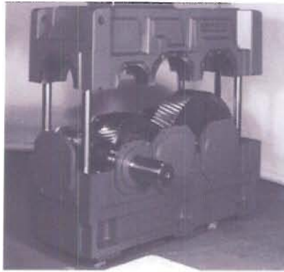
Figure 14: Wind Turbine Transmission
