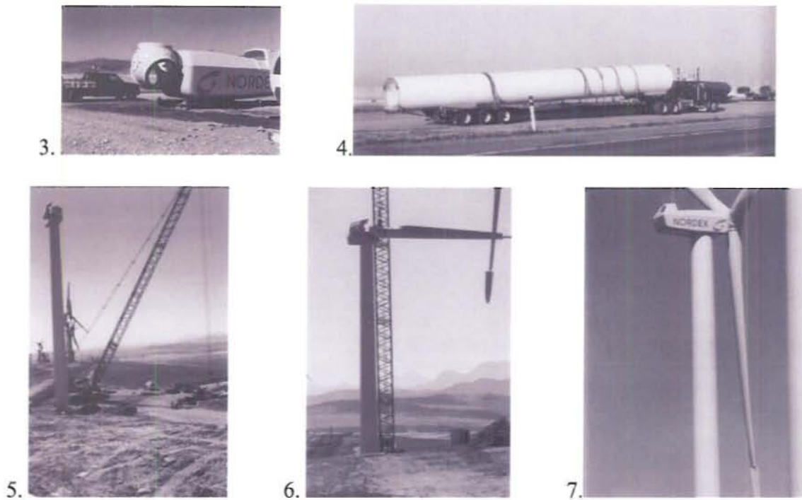
Figure 22: Turbine Construction Process [19]
