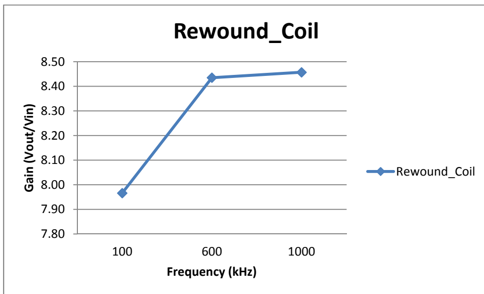
Figure 39: Rewound Coil's Frequency Response
