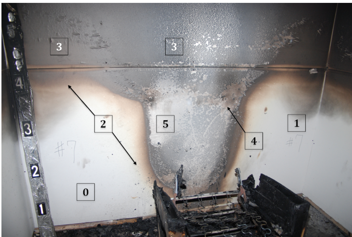
FIG. B-1 – Photograph from which selected images of visible damage indicators was chosen for use with the DOFD Method.
