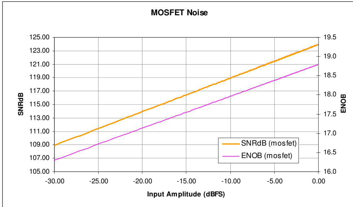
Figure 2-3 MOSFET Noise
