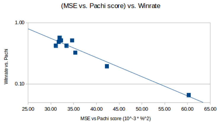
Figure 3.12: MSE (Policy vs Pachi score) vs Winrate. Winrate shown on logarithmic scale.
