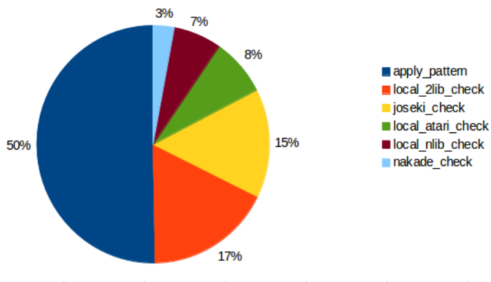
Figure 3.4: Time distribution of subpolicies in Seqchoose
