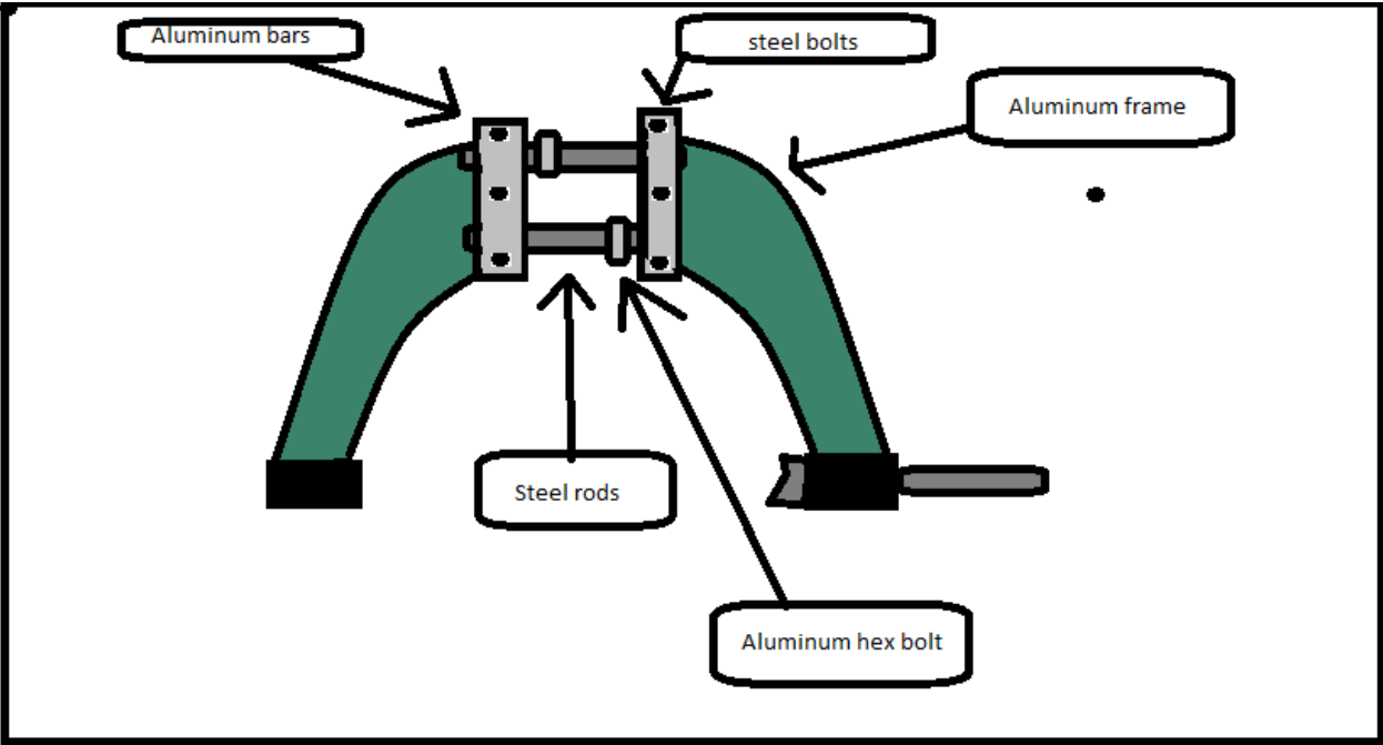
Figure 20: Gage Prototype Design
