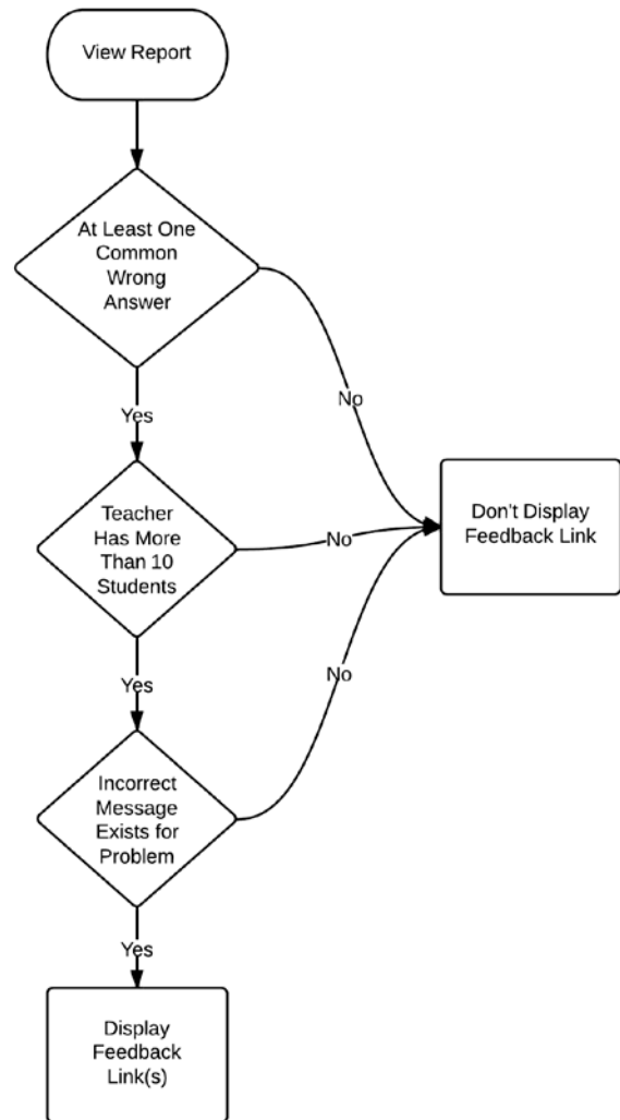
Figure 1: Basic flow of the incorrect message feature for reports
