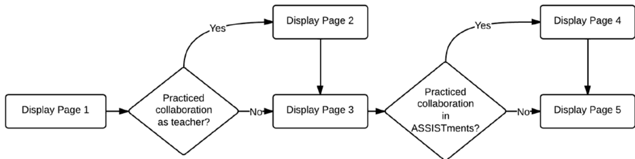
Figure 18: Flow of Collaboration Survey
