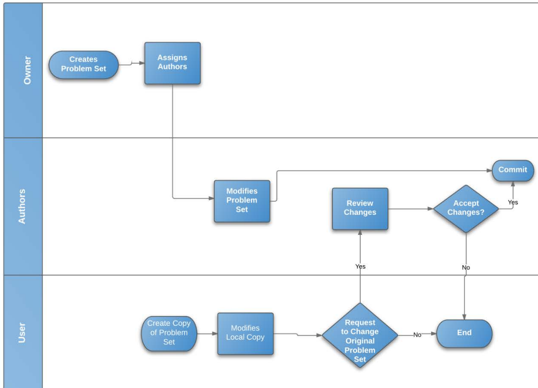
Figure 12: Interaction between user states and flow of modifying a problem set
