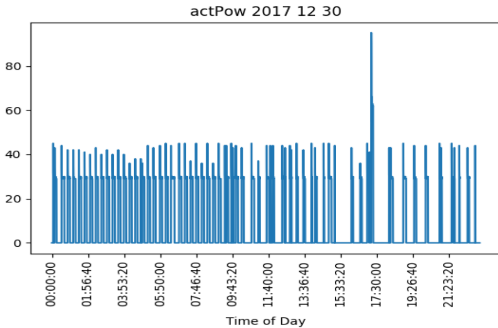
Figure 4.10b: Actual Power in HMO 2
