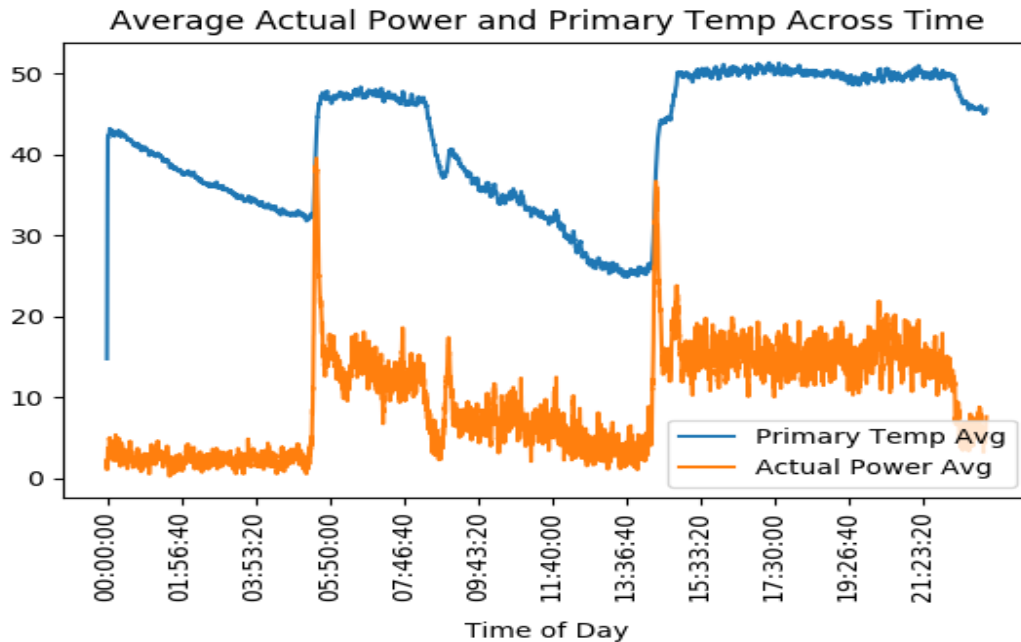
Figure 4.12b: Average Primary Temperature and Actual Power in HMO1
