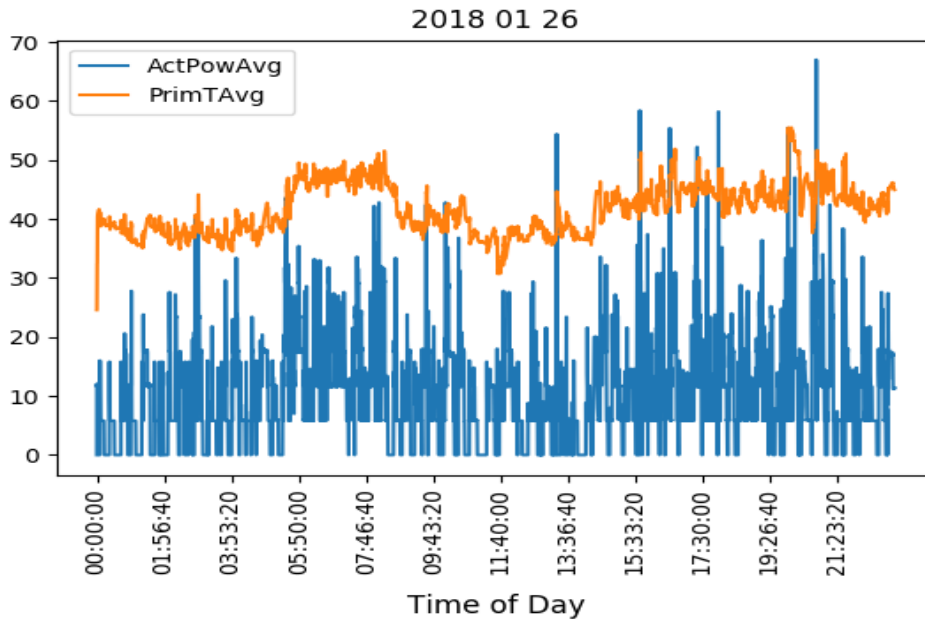
Figure 4.14b: Average Actual Power and Primary Temperature across five HMOs on 1/26/2018
