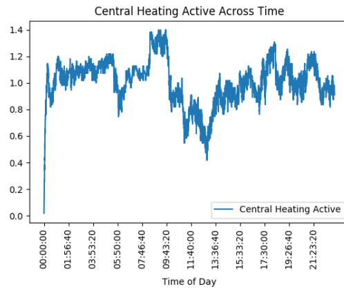
HMO4 Central Heating Active Across Time
