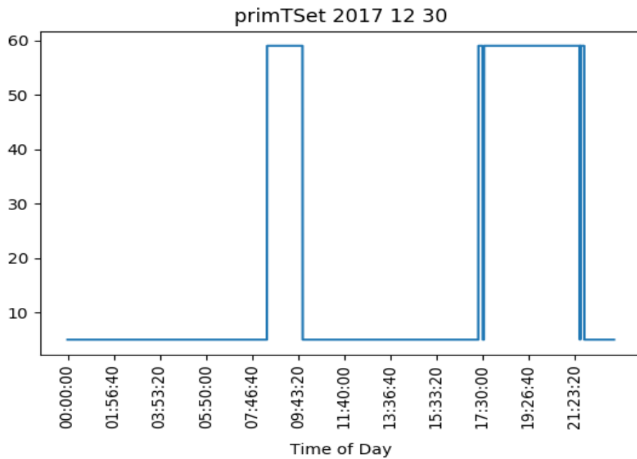
Figure 4.11a: Primary Temperature Setpoint in HMO1
