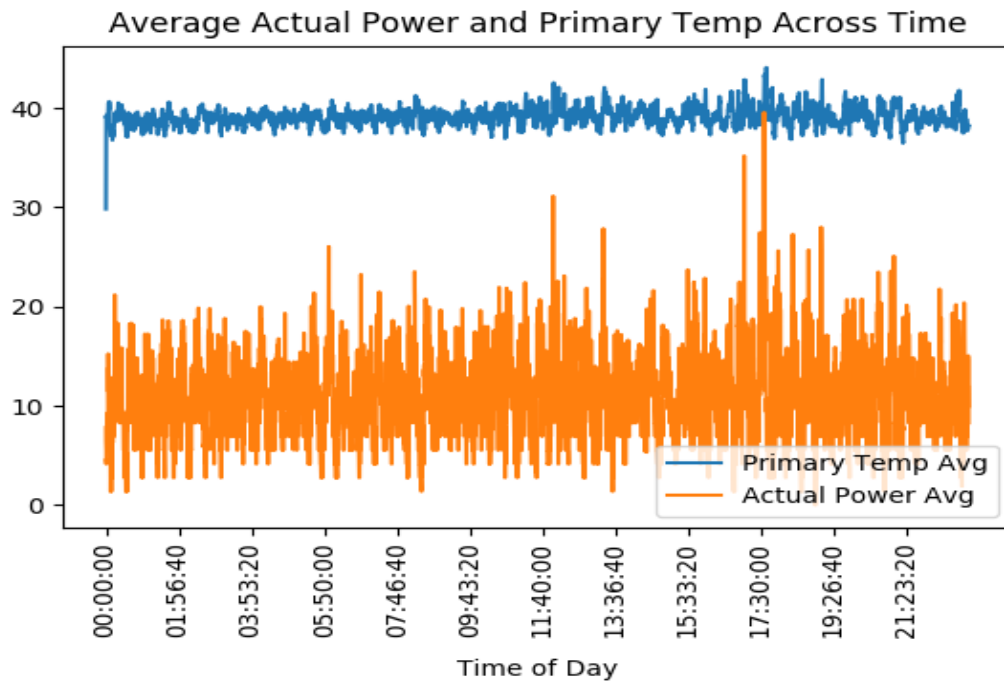
Figure 4.13b: Average Primary Temperature and Actual Power in HMO 2
