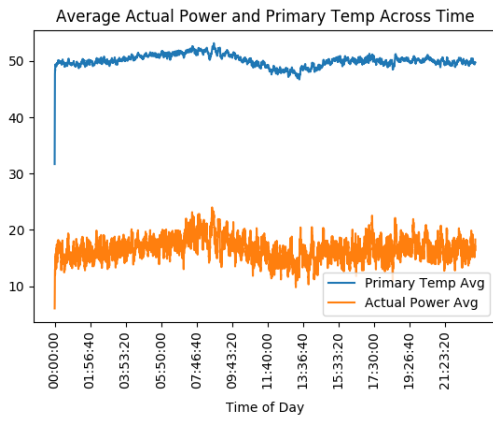
HM05 Average Actual Power and Primary Temperature Across Time
