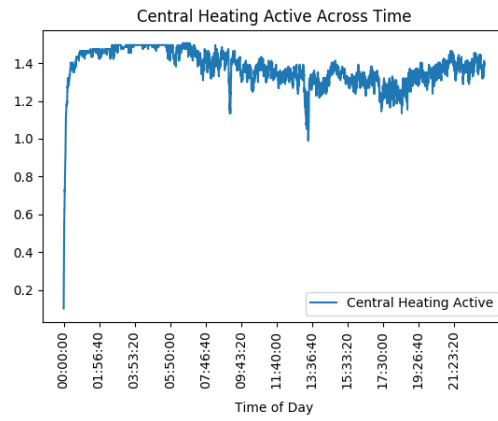
HM05 Central Heating Active Across Time
