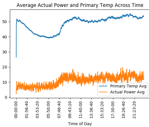
HMO3 Average Actual Power and Primary Temperature Across Time
