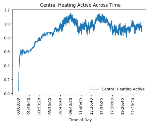
HMO3 Central Heating Active Across Time
