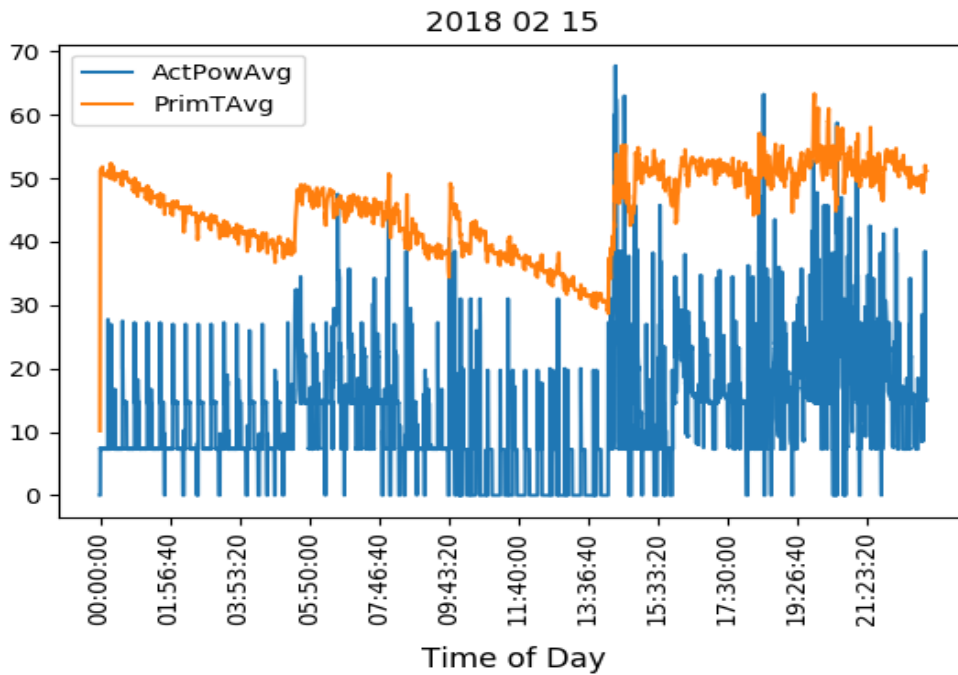
Figure 4.15b: Average Actual Power and primary temperature across four HMOs 02/15/2018
