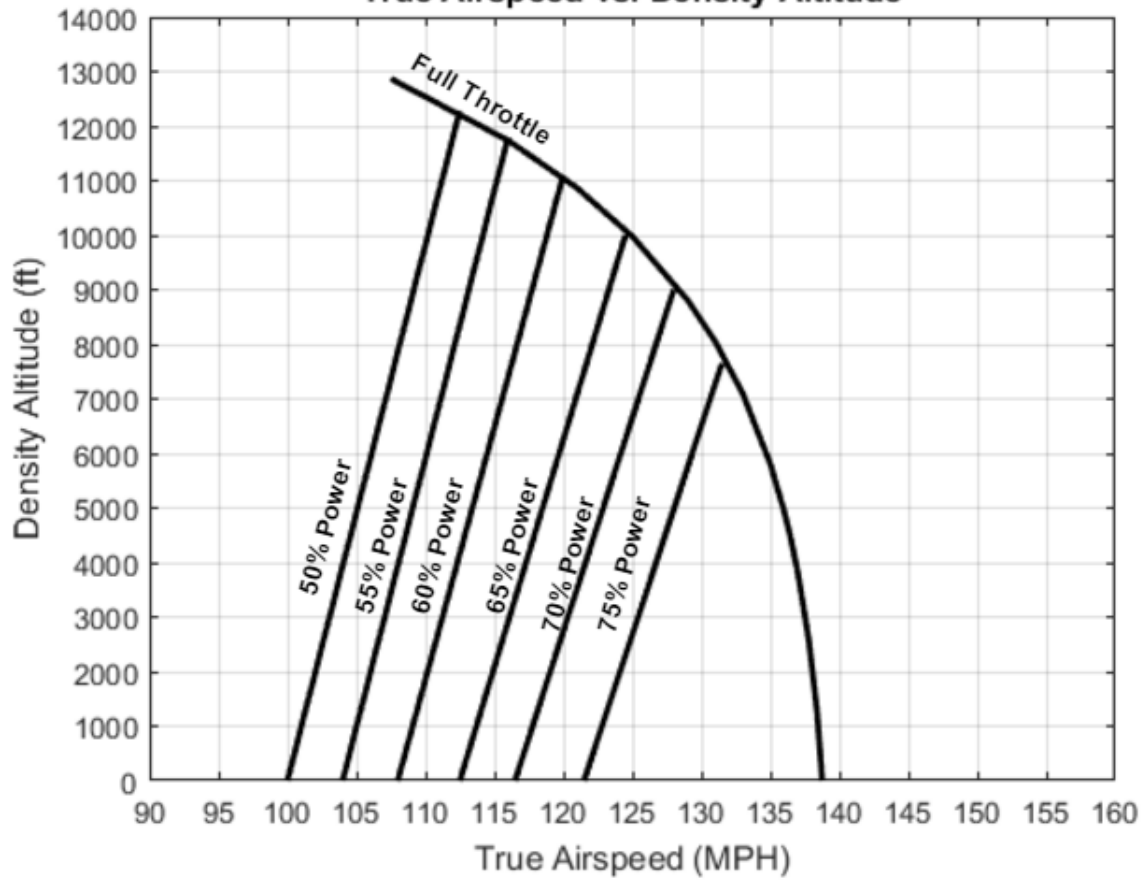
True Airspeed vs. Density Altitude
