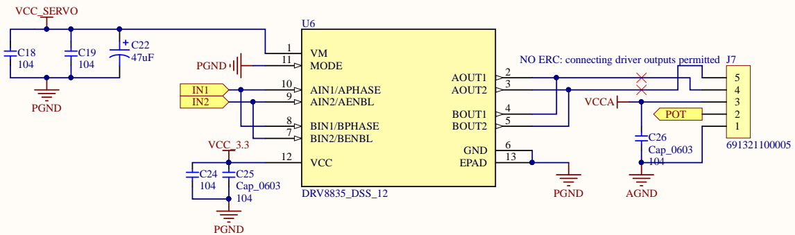
Figure D.11: Clutch servo driver circuit
