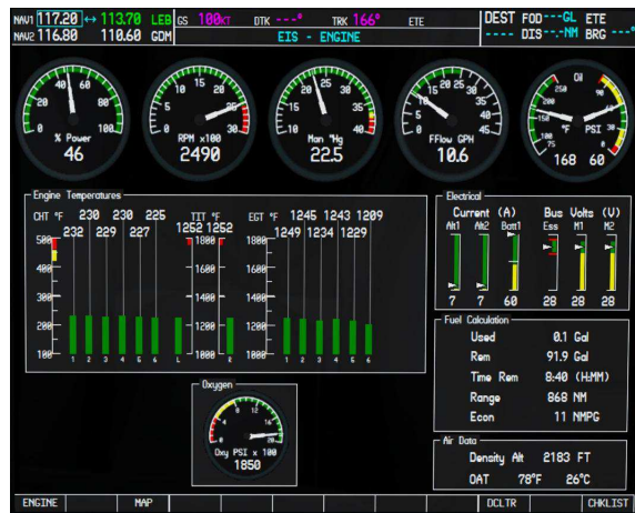
Figure F19: Garmin G1000 Secondary Display
