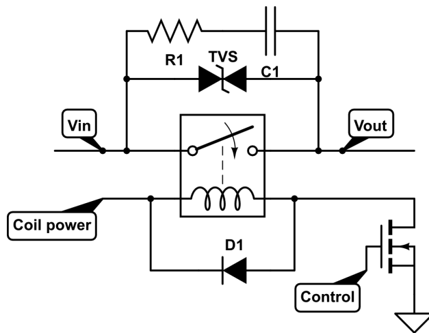
Figure D.9: Relay arc suppression circuit
