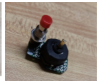
Figure B11: Shrink Wrap around the 5-way switch
