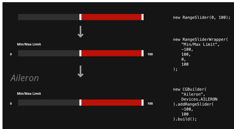
Figure F12: Control Group Builder Flow Diagram
