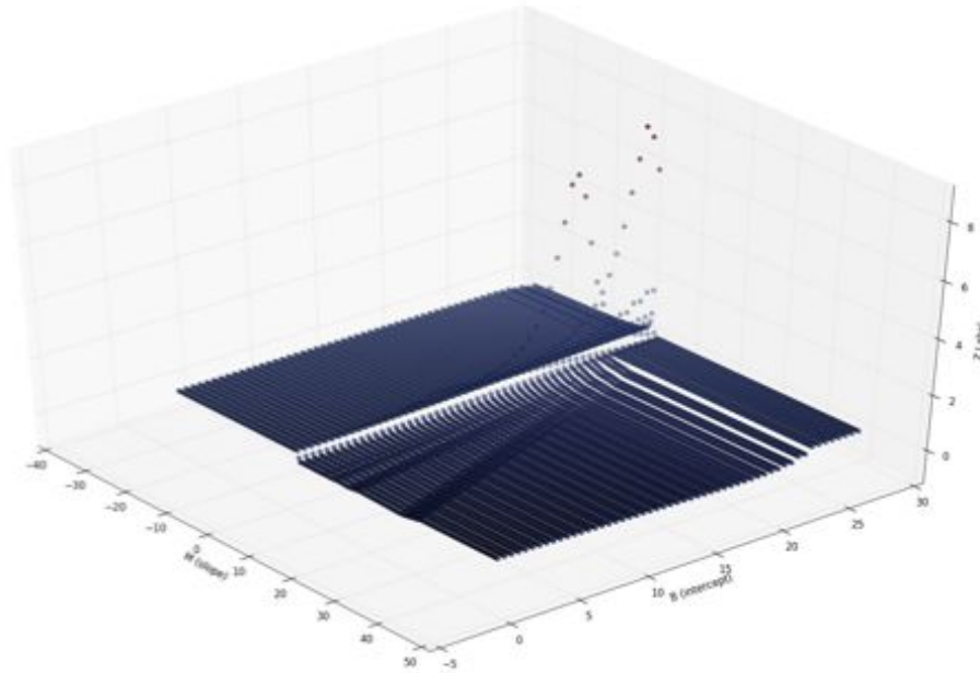
Figure 15: The algorithm running on an artificially rotated stock photo (top) with the detected horizon in red, and the cost function surface (here in transformed Slope-Intercept space instead of pitch-bank space)
