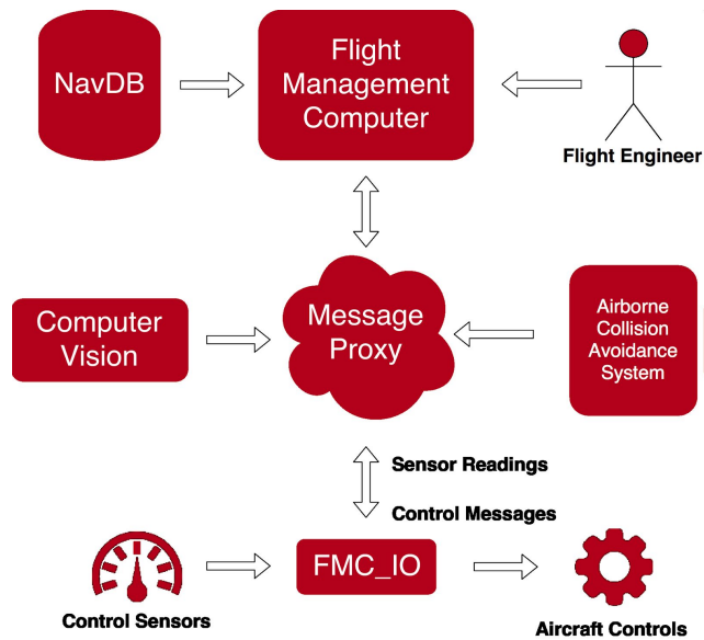
Figure 9: Software Architecture
