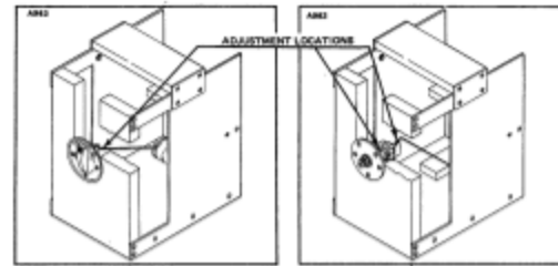
Figure 9-6. Fuel Quantity Transmitter (P/N 62037-00)
