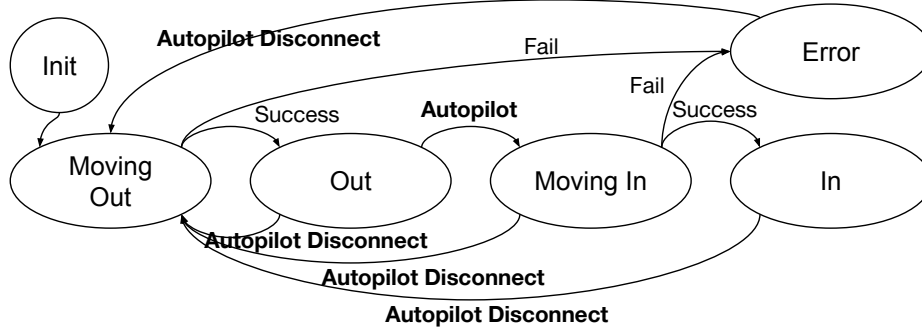
Figure D.8: State transition diagram of clutch servo motors
