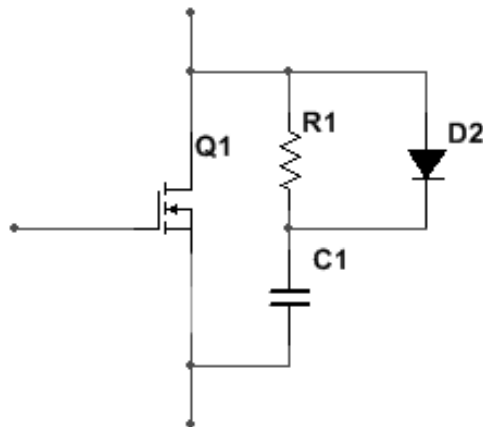
Figure 4.5: Ideal Snubber
