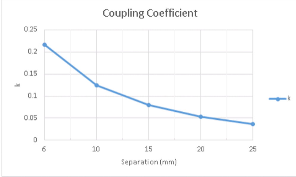
Figure 4.6: Simulation results
