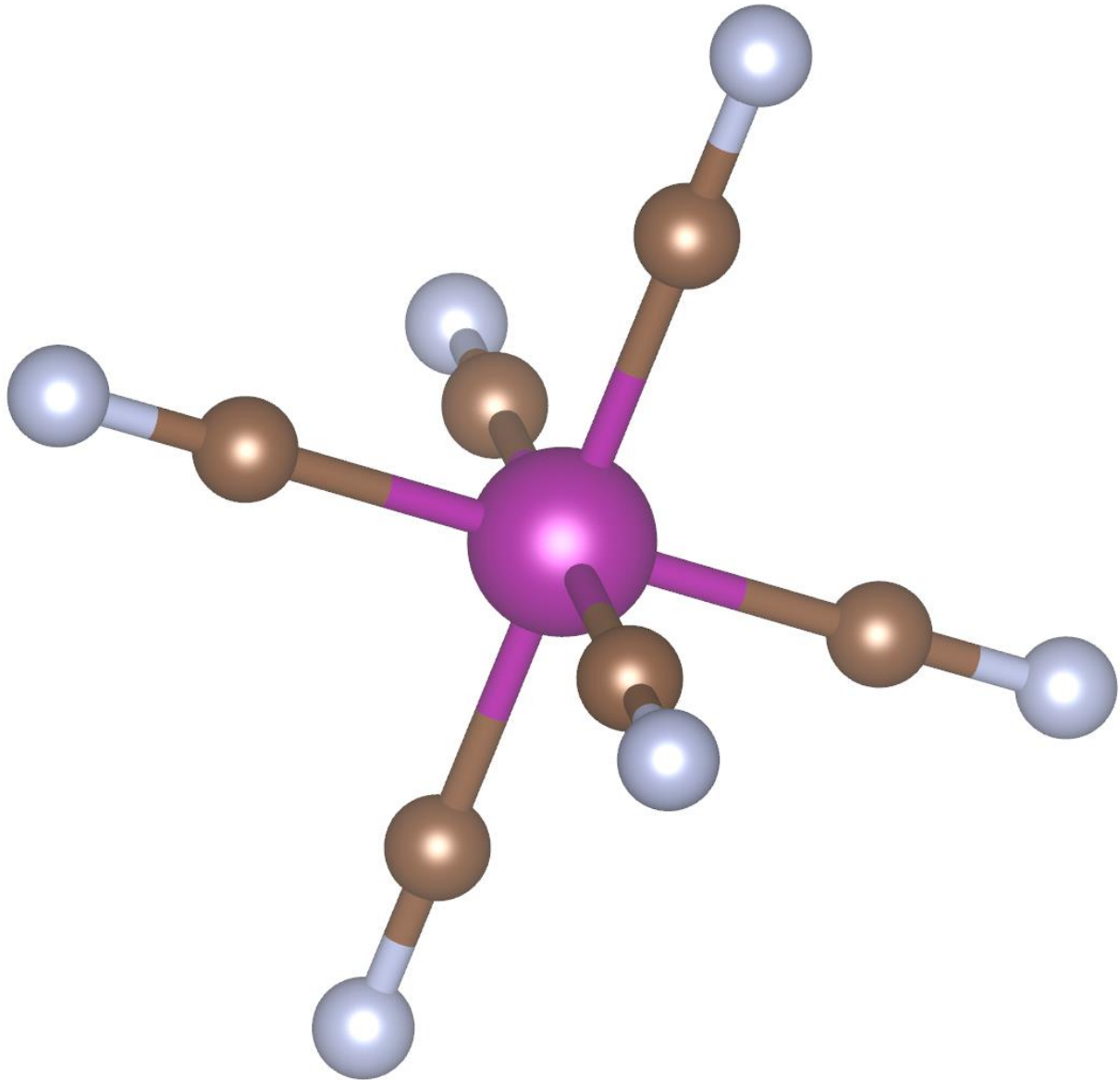
Figure B3: \text{Mn}(\text{CN})_6^{4-} , Hexacyanomanganate.
