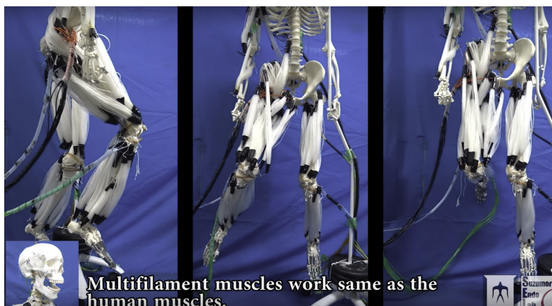
Figure 3.2.: Pneumatically-operated artificial muscles controlling skeletal limbs [9].
