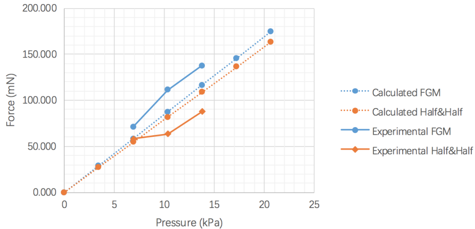
Figure 5.12.: Plot of Force vs. Pressure Results for Each of the Actuators.
