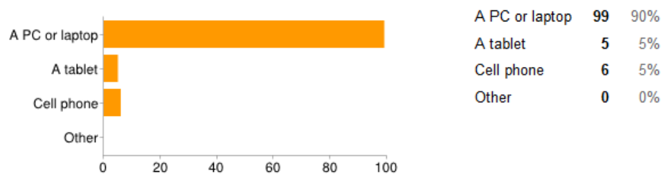
Figure 19: Device Statistics
