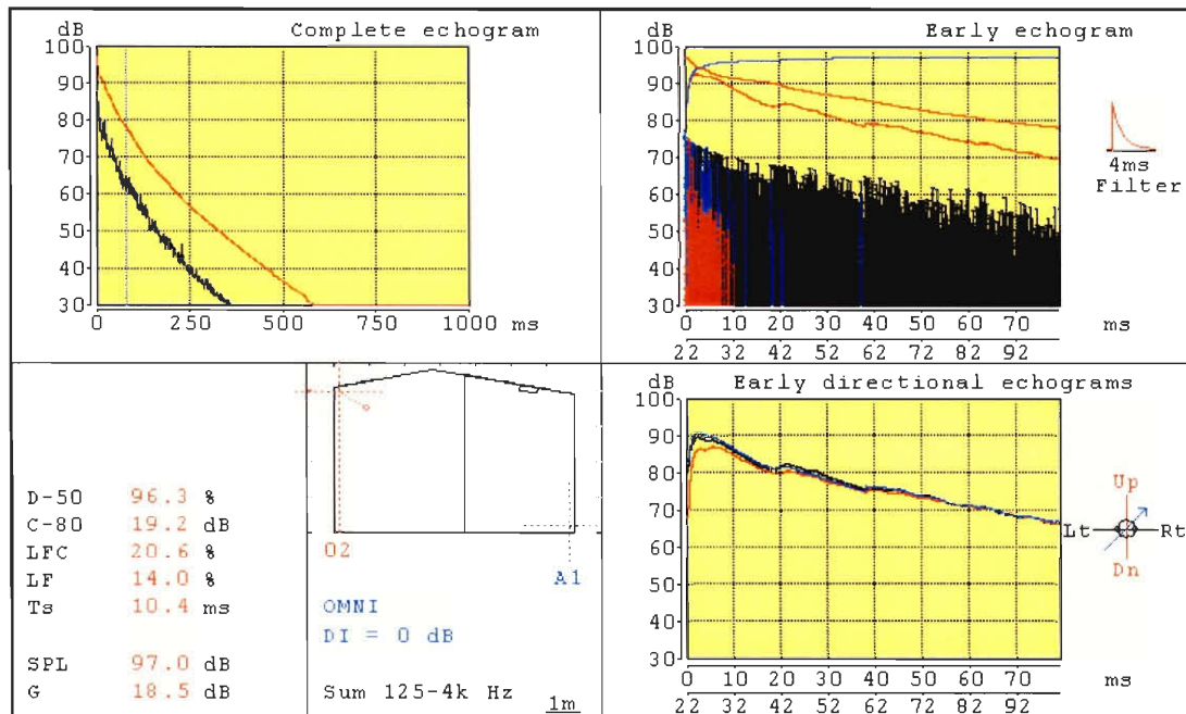
Figure 23 Echogram for source A1 and receiver 02
