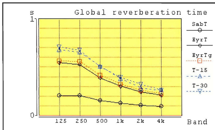
Figure 10 Global reverberation time simulated for WICN's Performance Room in its current state (carpeting and Celotex panels present in space)
