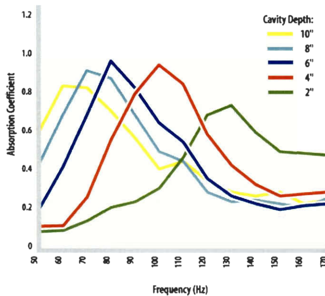
Figure 18 Modex Absorption Coefficients xvii
