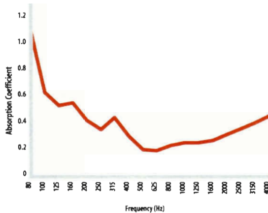
Figure 17 Modex Corner absorption coefficients in effective range xvii
