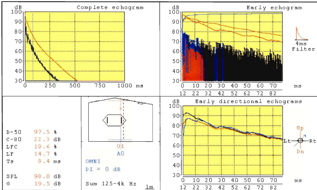
Figure 22 Echogram for source A0 and receiver 01
