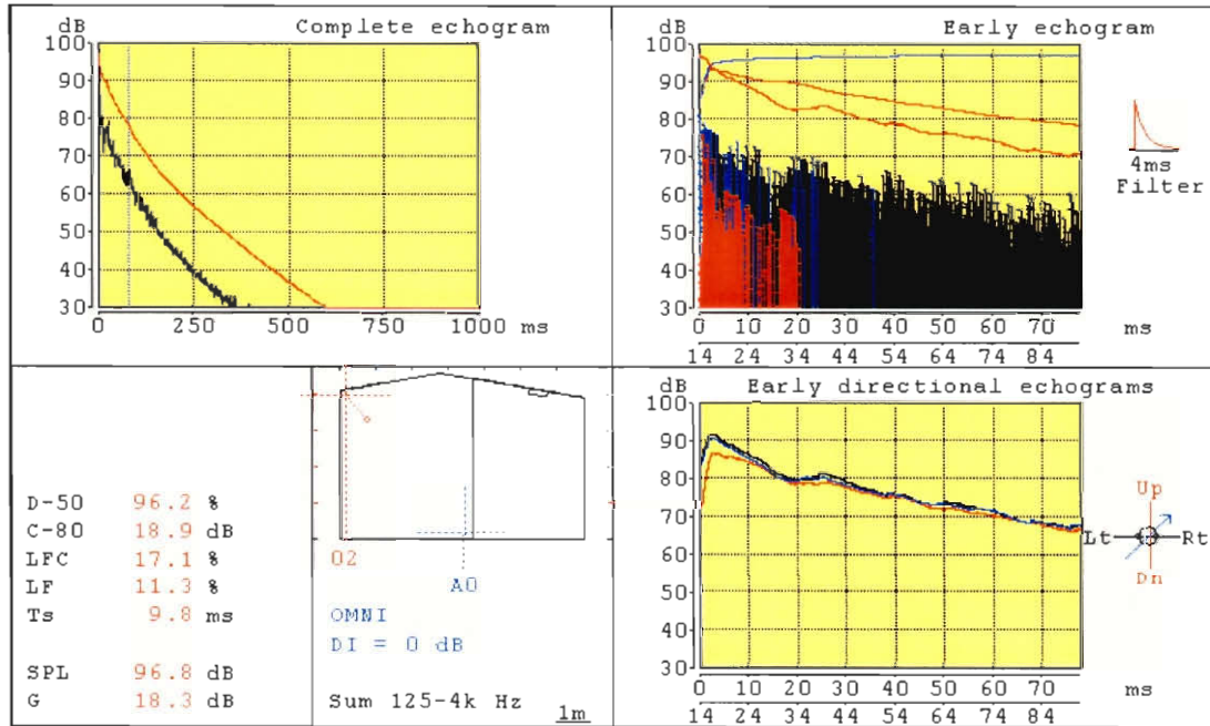
Figure 25 Echogram for source A0 and receiver 02
