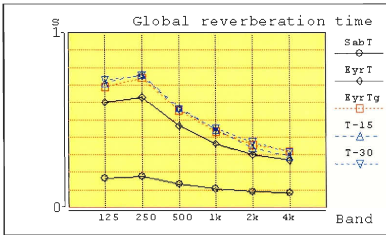
Figure 16 Global reverberation time after implementing the stage
