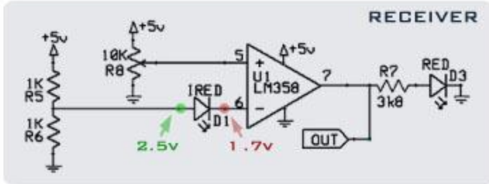
LOW RANGE, ALWAYS ON IR PROXIMITY SENSOR DESIGNED BY IBRAHIM KAMAL - IKA@IKALOGIC.COM
